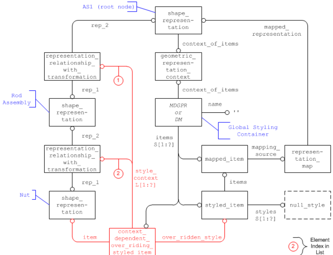
Figure 13: Styling an instance of a component in an assembly
