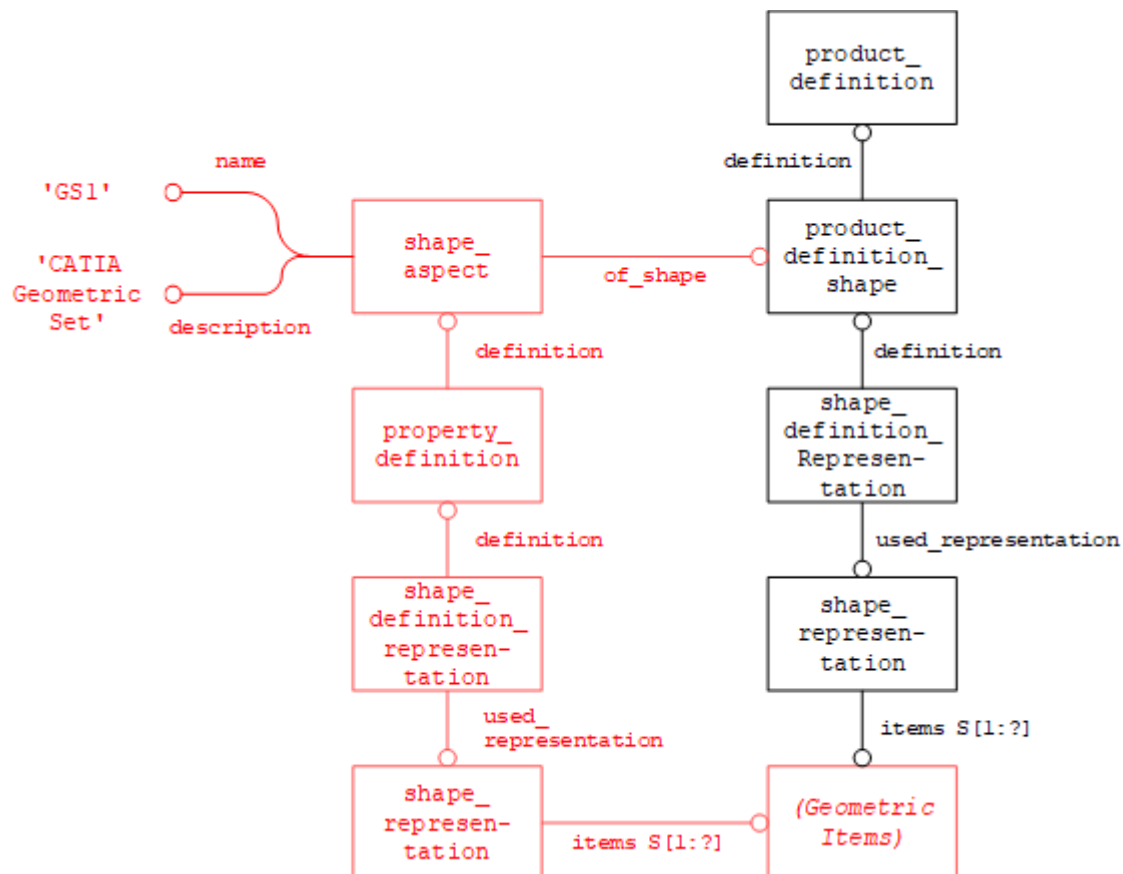
Figure 19: Defining Geometry for CATIA Geometric Sets
