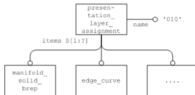
Figure 15: Layer Representation
