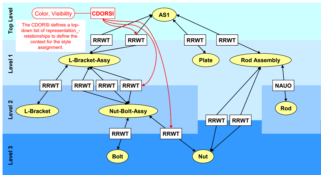
Figure 12: Identification of the Instance to be styled
