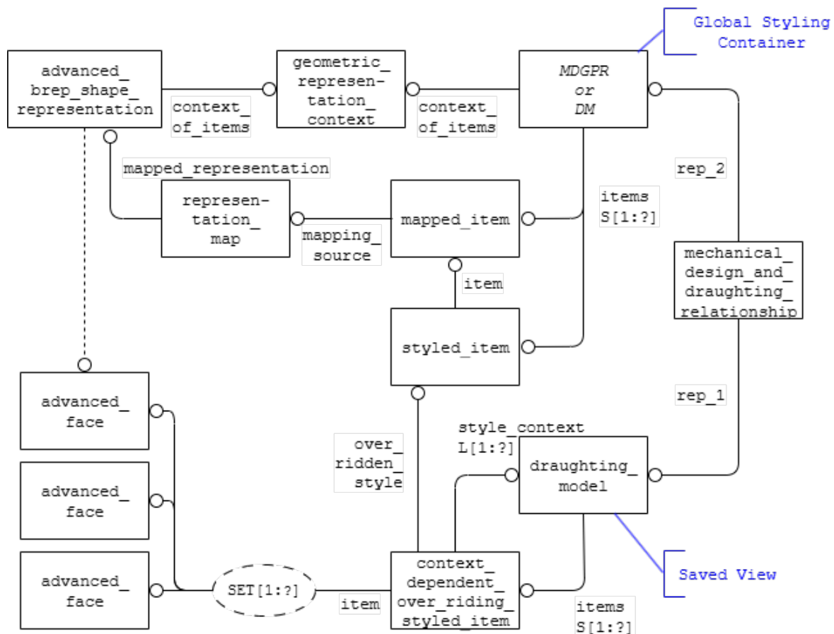
Figure 11: Styling several Items at Once
