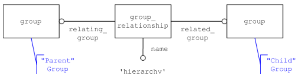
Figure 17: Group Relationship Representation
