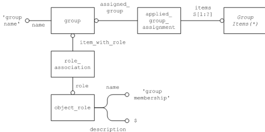
Figure 16: Group Assignment Representation
