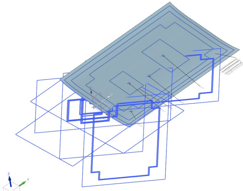
Figure 6: Illustration of the “Laminate Plate” model (NX)
