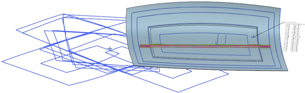
Figure 7: Illustration of the “Sandwich Plate” model (NX)
