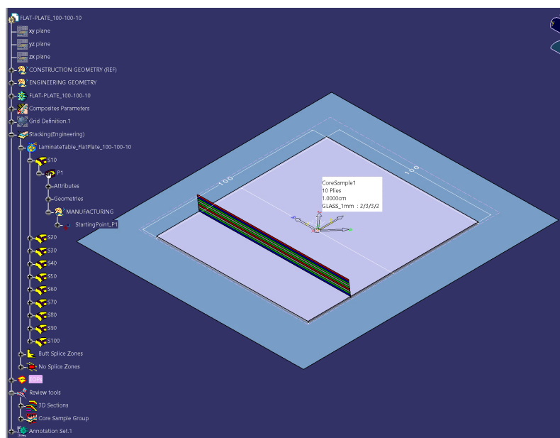
Figure 5: Illustration of the “Flat Plate” model (CATIA V5, Creo)
