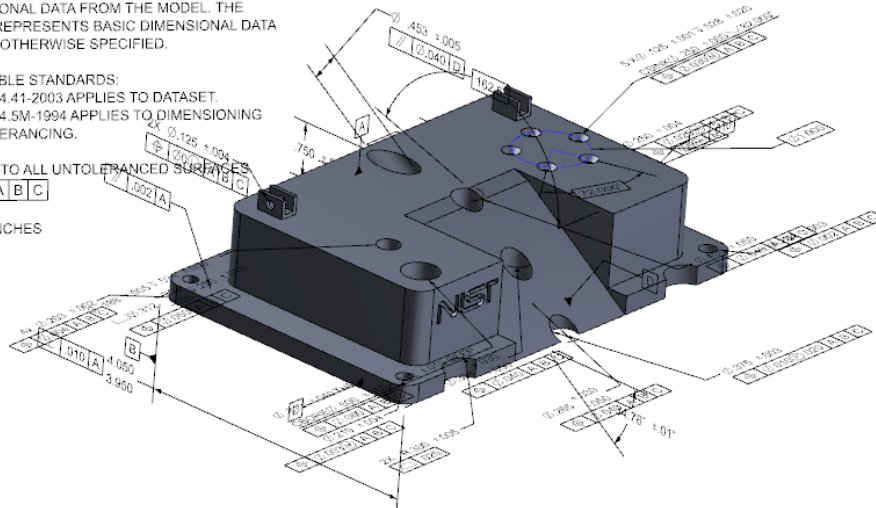
Figure 6: View of the PDC model for the HTC test case with all annotations switched on
