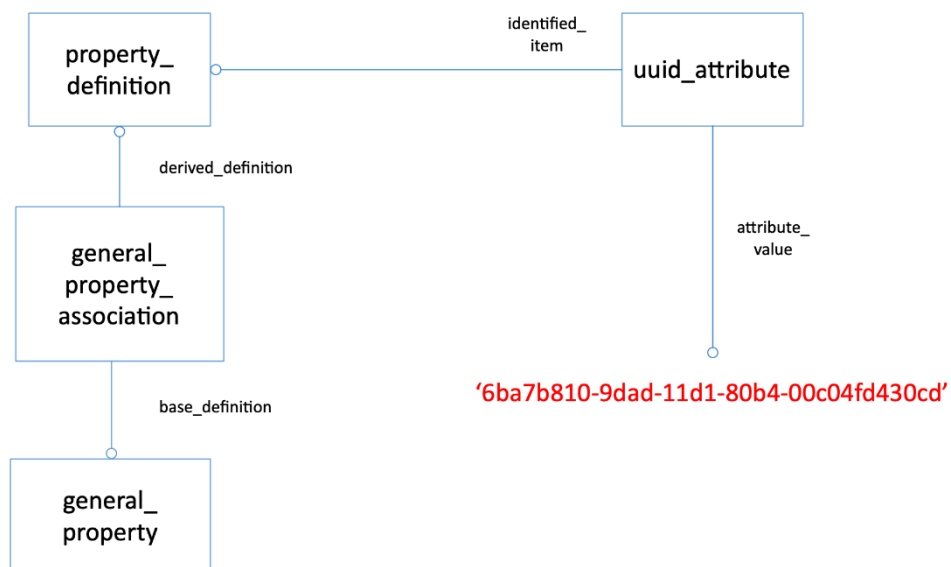
Figure 10: Entity Identifier for UDA
