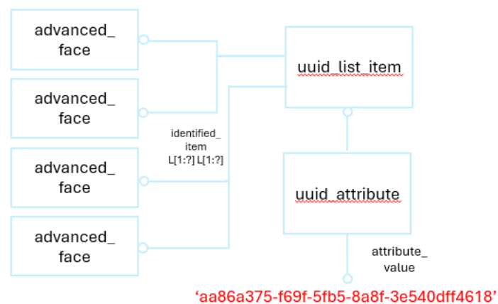
Figure 8b: Entity Identifier using uuid_list_item for Topology/Geometry (note – uuid_attribute must be replaced by either v5_uuid_attribute or v4_uuid_attribute.)
