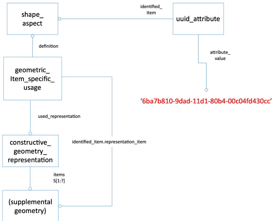
Figure 9: Entity Identifier for Supplemental Geometry
