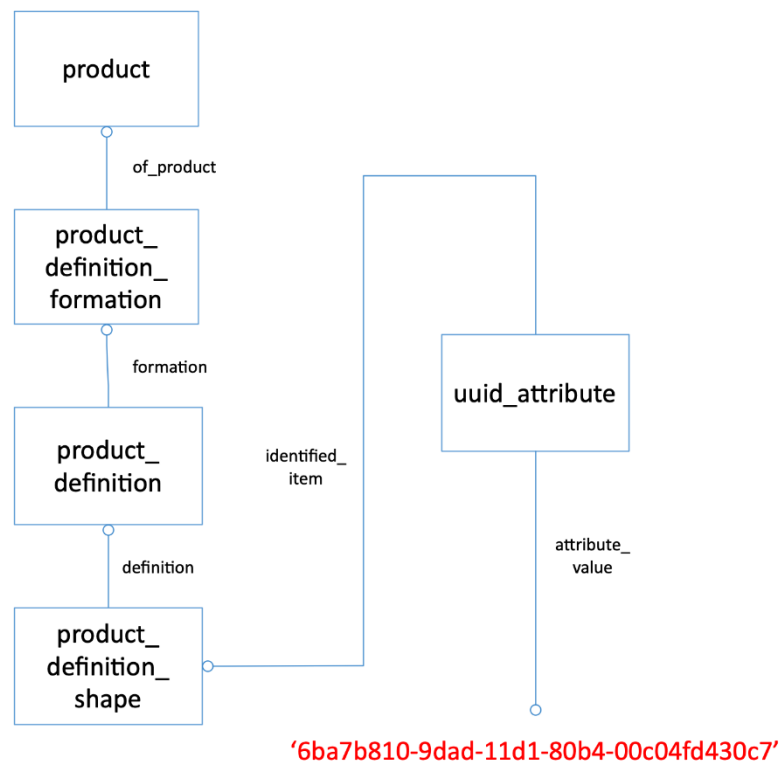
Figure 6: Entity Identifier for Product
