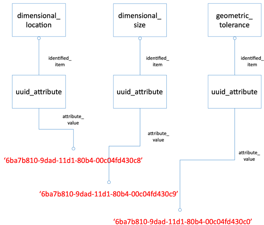
Figure 7: Entity Identifiers for PMI (examples) (note – uuid_attribute must be replaced by either v5_uuid_attribute or v4_uuid_attribute .)
