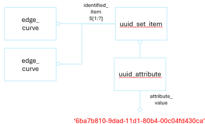
Figure 8a: Entity Identifier using uuid_set_item for Topology/Geometry (note – uuid_attribute must be replaced by either v5_uuid_attribute or v4_uuid_attribute .)
