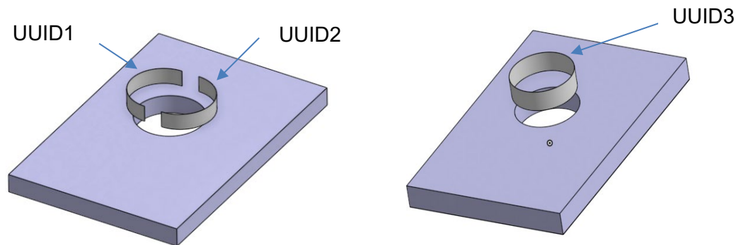
Figure 3a - Preprocessor - Half Cylinders Figure 3b - Postprocessor - Single Cylinder
