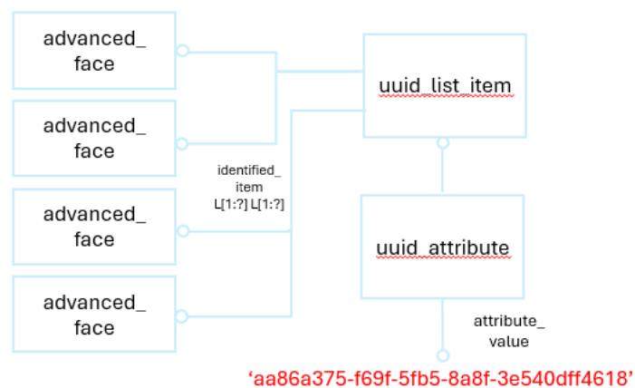
Figure 9b: Entity Identifier using uuid_list_item for Topology/Geometry (note – uuid_attribute must be replaced by either v5_uuid_attribute or v4_uuid_attribute .)
