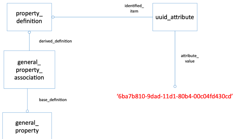
Figure 11: Entity Identifier for UDA
