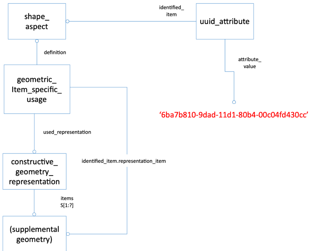
Figure 10: Entity Identifier for Supplemental Geometry
