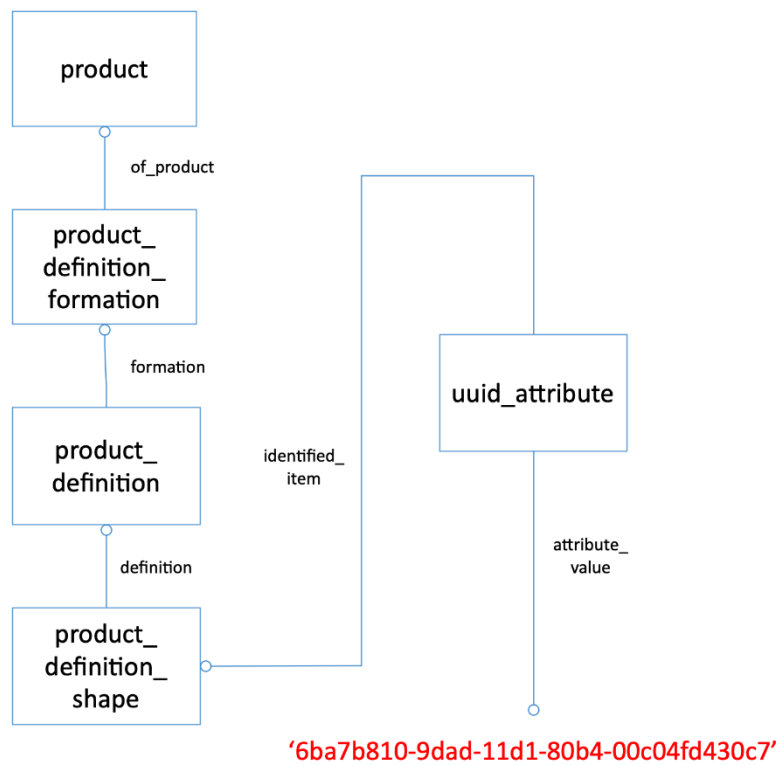
Figure 6: Entity Identifier for Product
