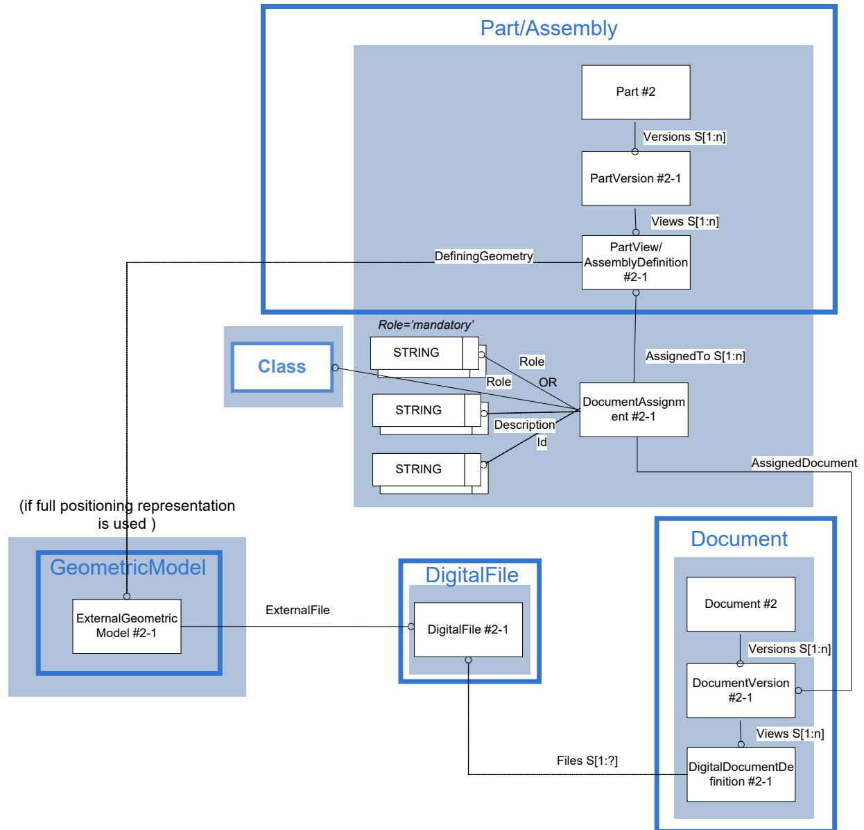
Figure 98: Template “PDM Representation for DocumentAssignment”
