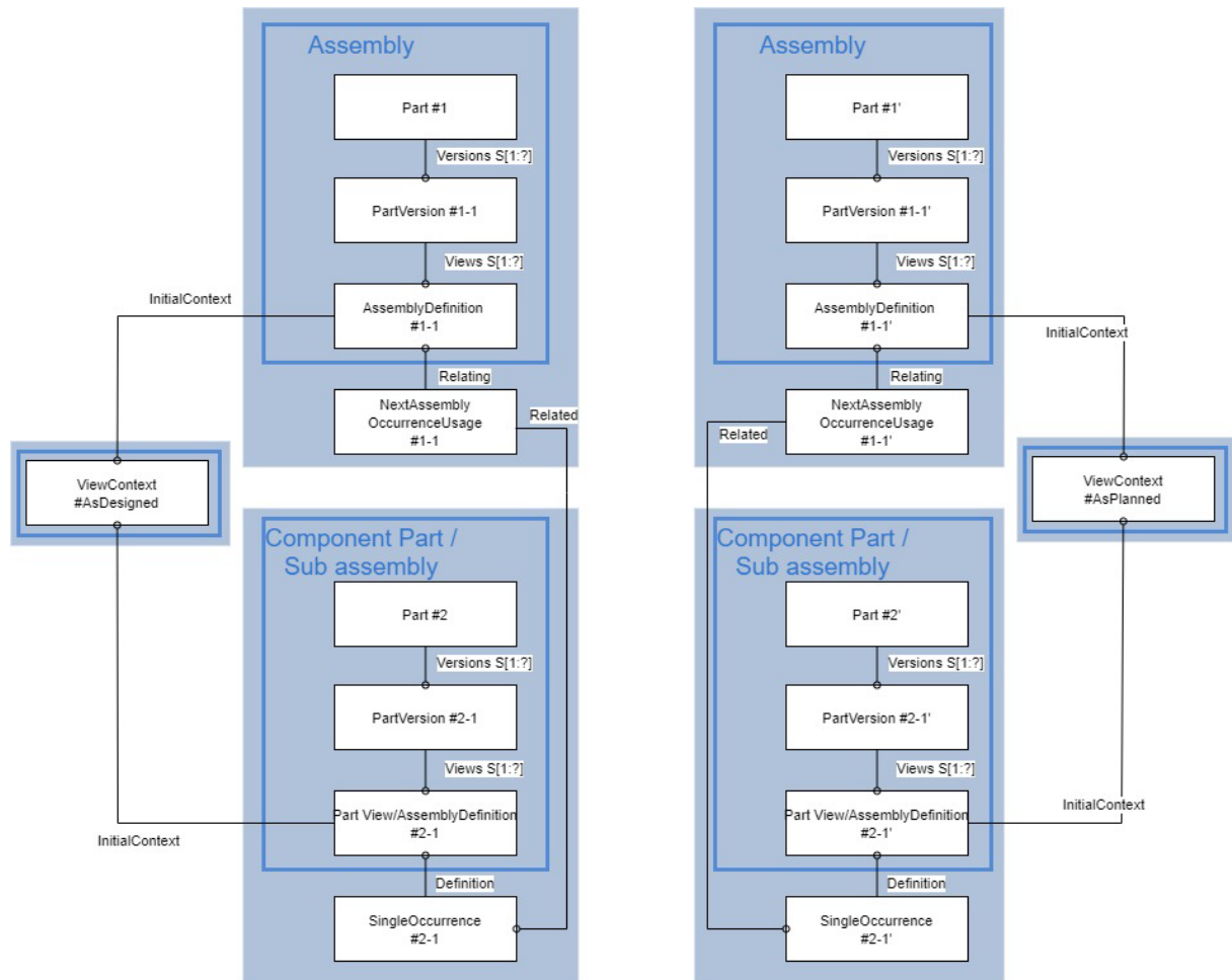
Figure 120: Representation of As Designed and As Planned views
