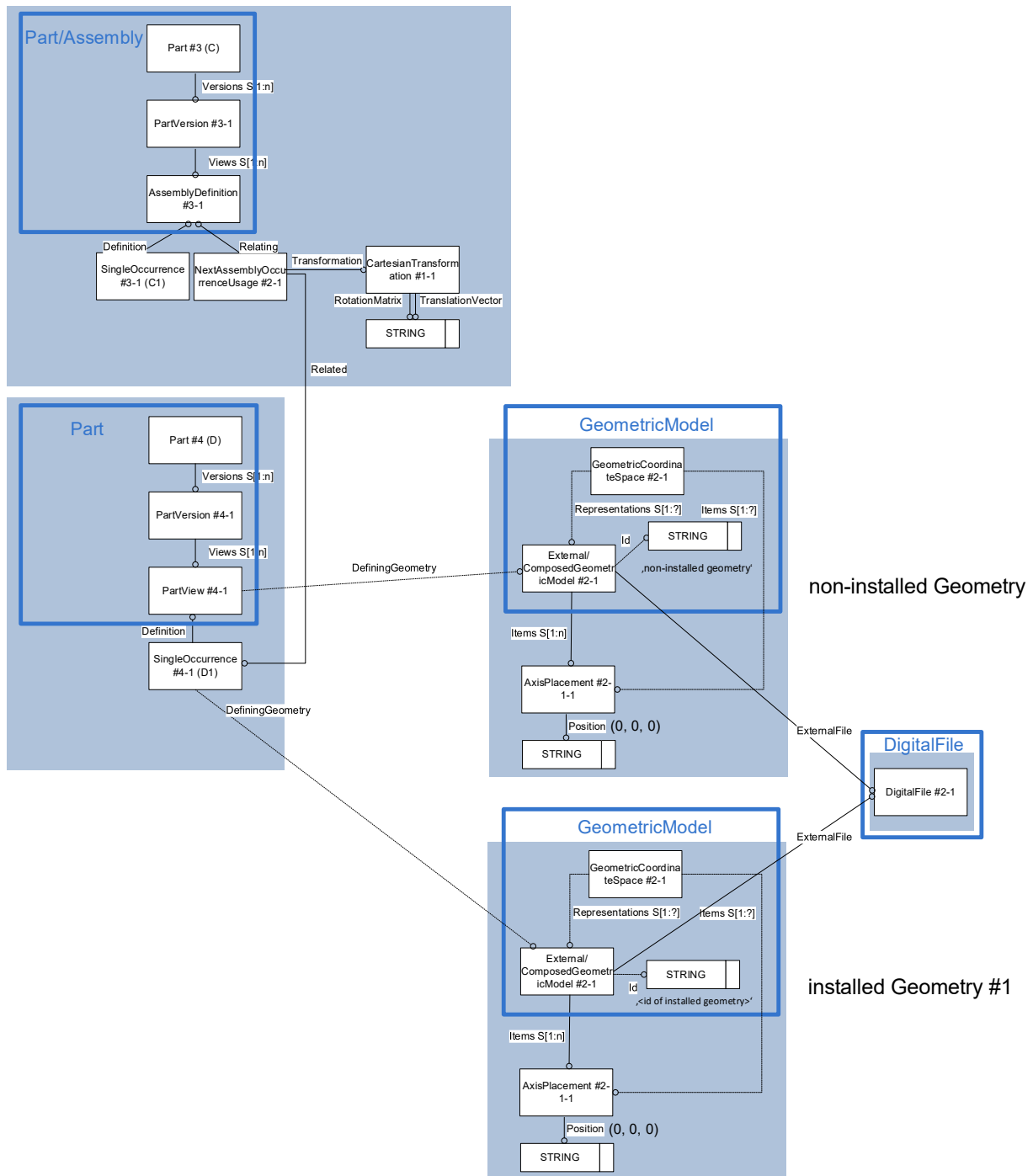
Figure 54: Example of alternative instance shapes
