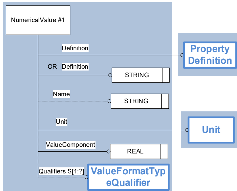
Figure 9: Template "NumericalValue"
