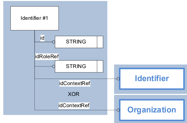
Figure 6: Template "Identifier"
