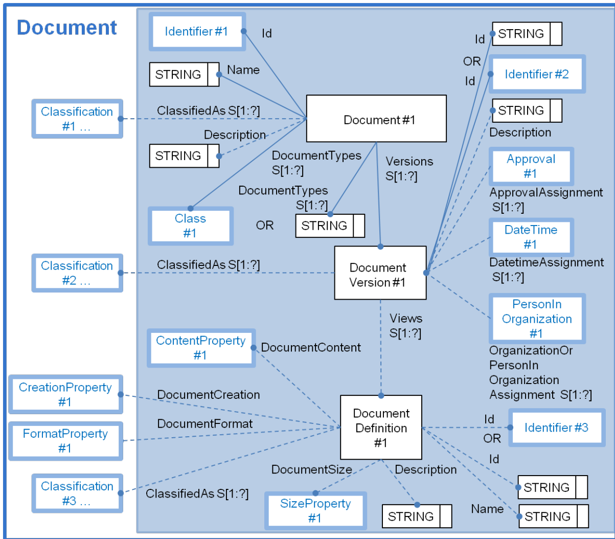
Figure 56: Template "Document"
