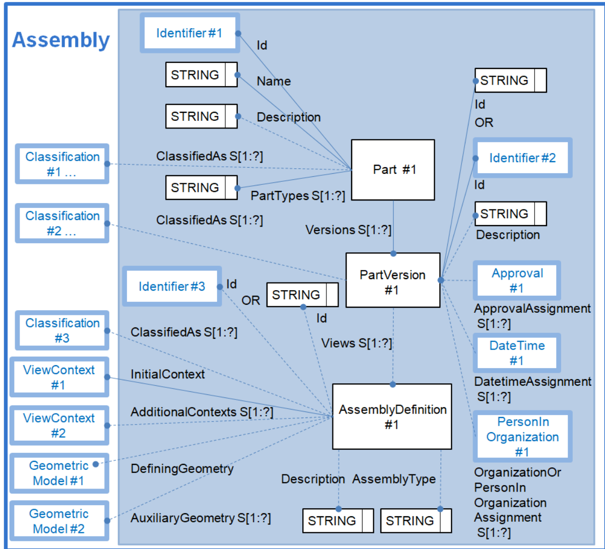
Figure 26: Template "Assembly"
