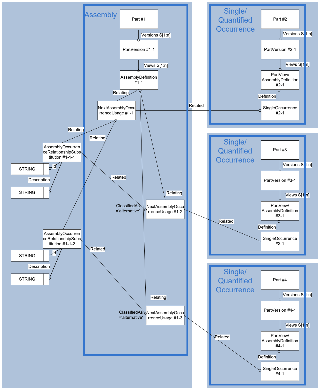
Figure 46: Template "AssemblyOccurrenceRelationshipSubstitution"
