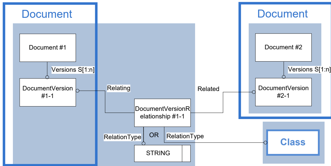
Figure 58: Template "DocumentVersionRelationship"
