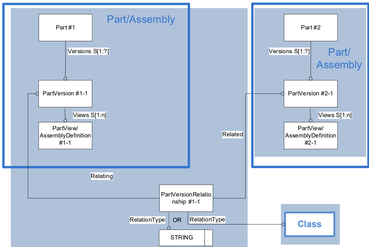
Figure 27: Template “PartVersionRelationship”
