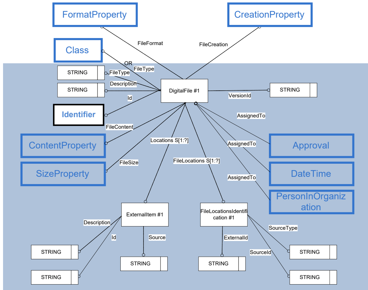
Figure 59: Template "DigitalFile"
