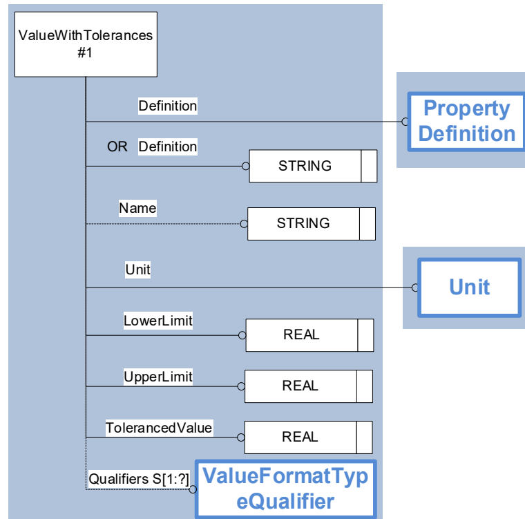
Figure 12: Template “ValueWithTolerances”
