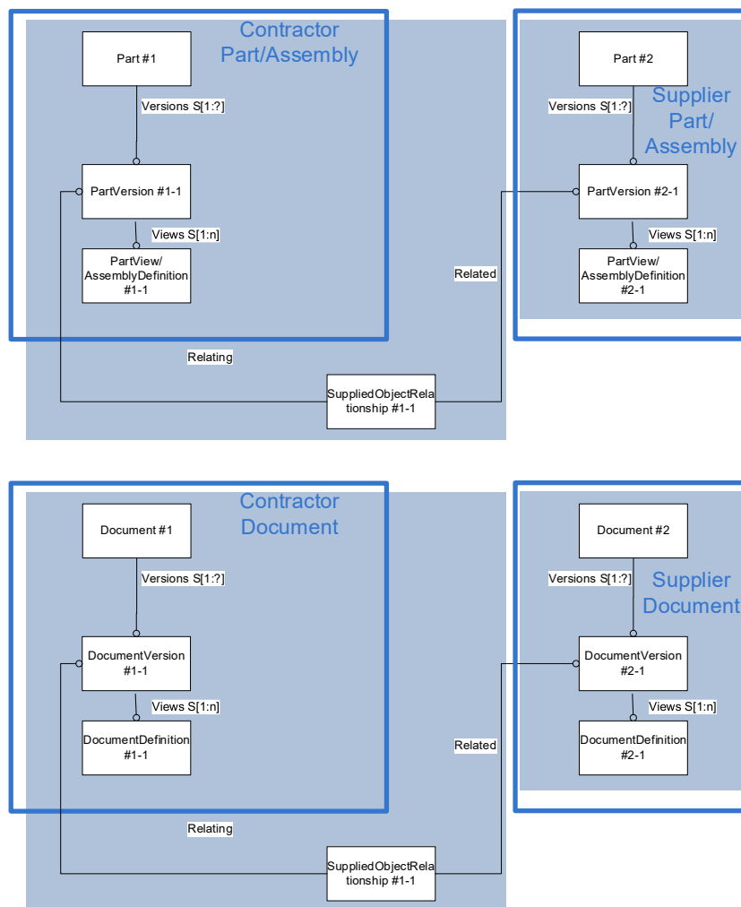
Figure 22: Template “SuppliedObjectRelationship”
