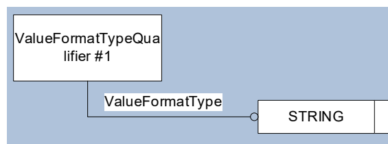
Figure 21: Template “ValueFormatTypeQualifier”
