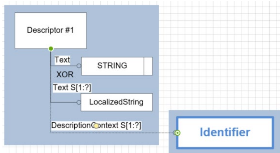
Figure 7: Template "Descriptor"
