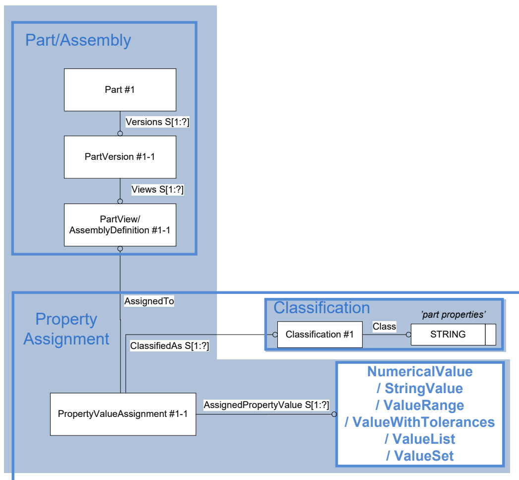
Figure 29: Template “PropertyAssignment”
