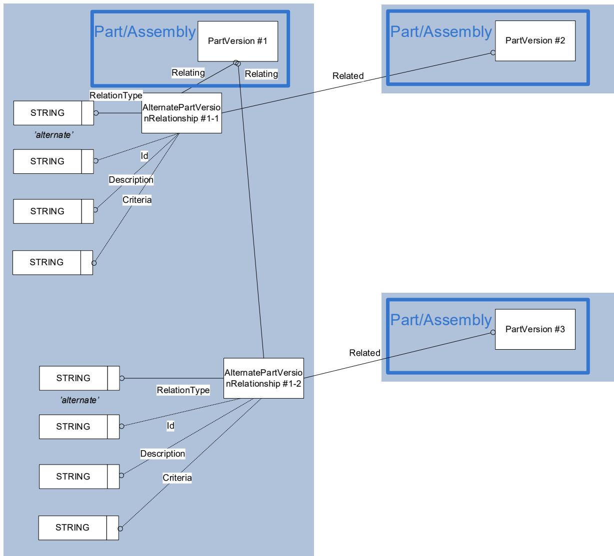
Figure 45: Template "AlternatePartVersionRelationship"
