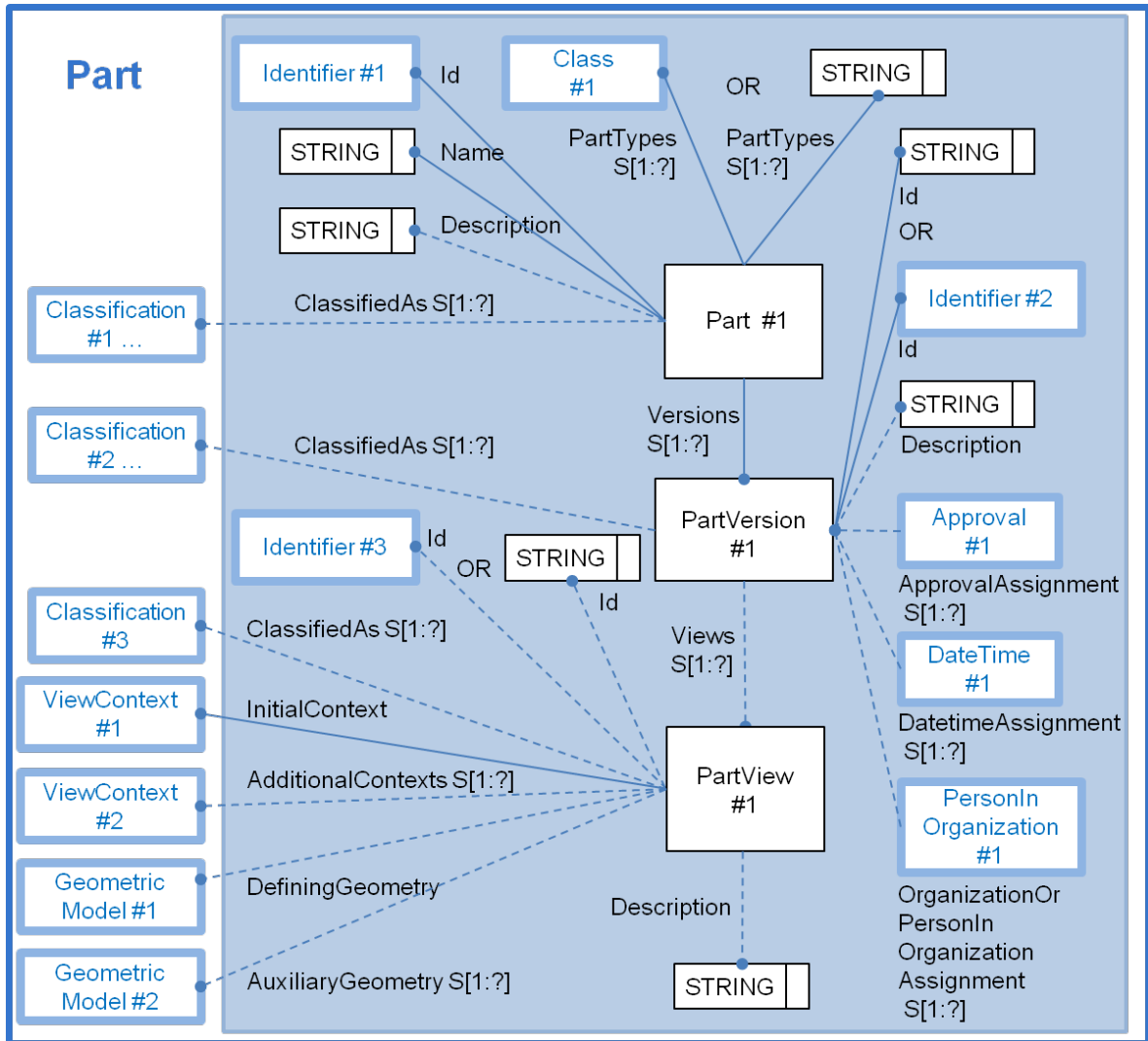
Figure 25: Template "Part"
