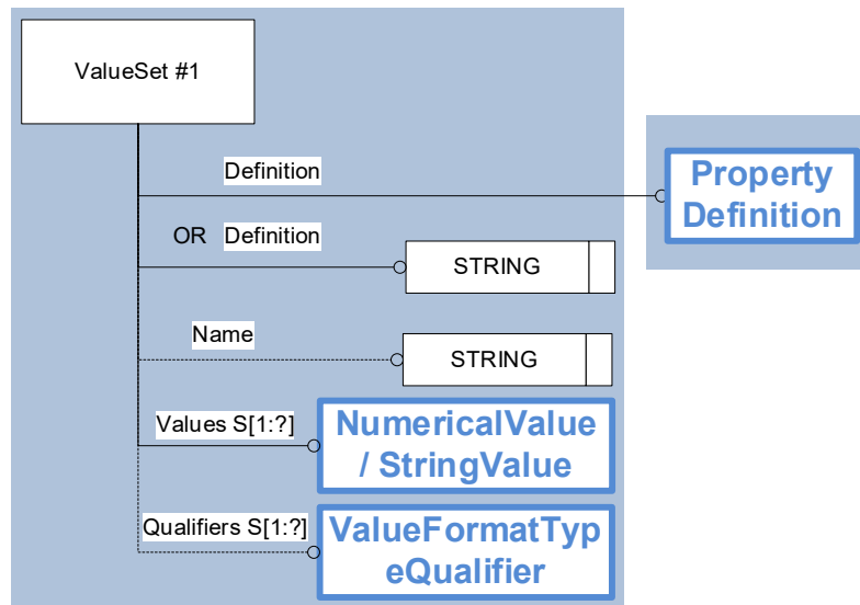
Figure 15: Template "ValueSet"
