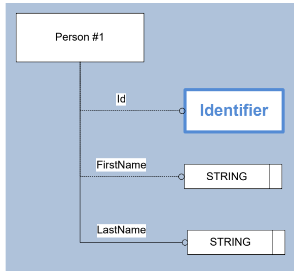
Figure 18: Template “Person”
