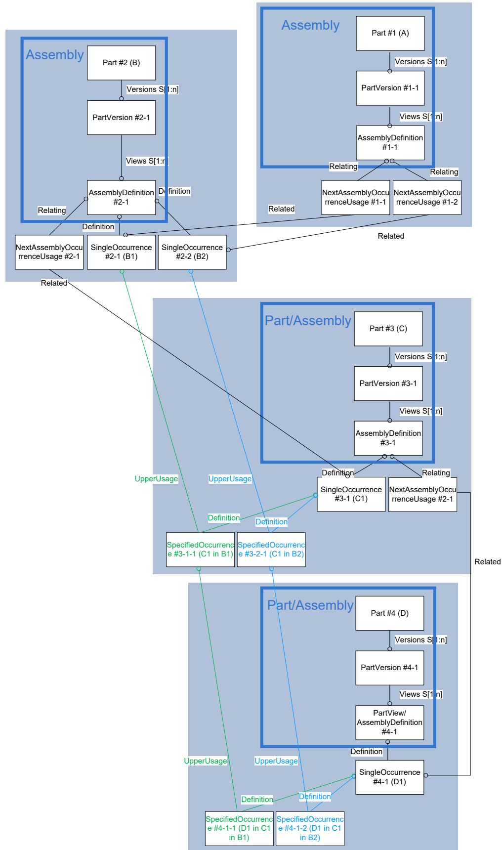
Figure 33: Template "SpecifiedOccurrence"
