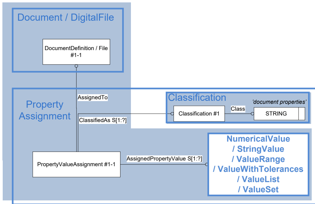
Figure 92: Template "DocumentFileProperty"
