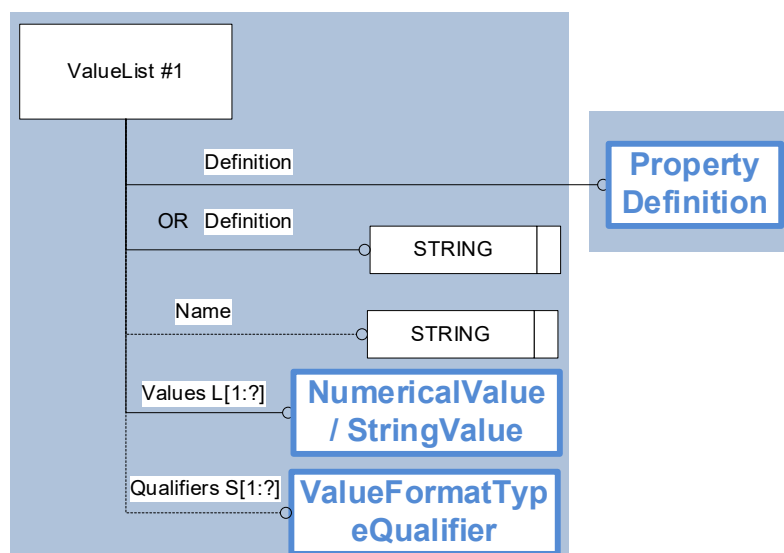
Figure 14: Template “ValueList”
