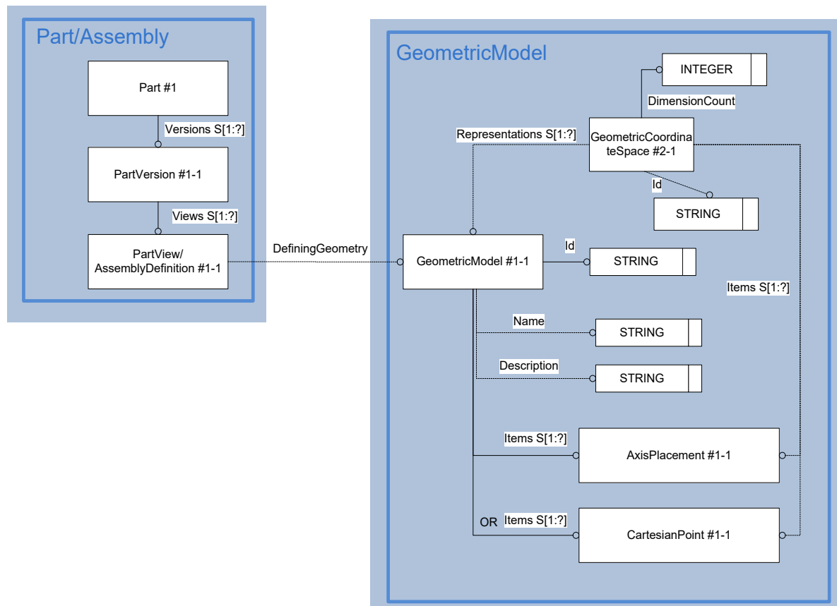
Figure 28: Template "GeometricModel"
