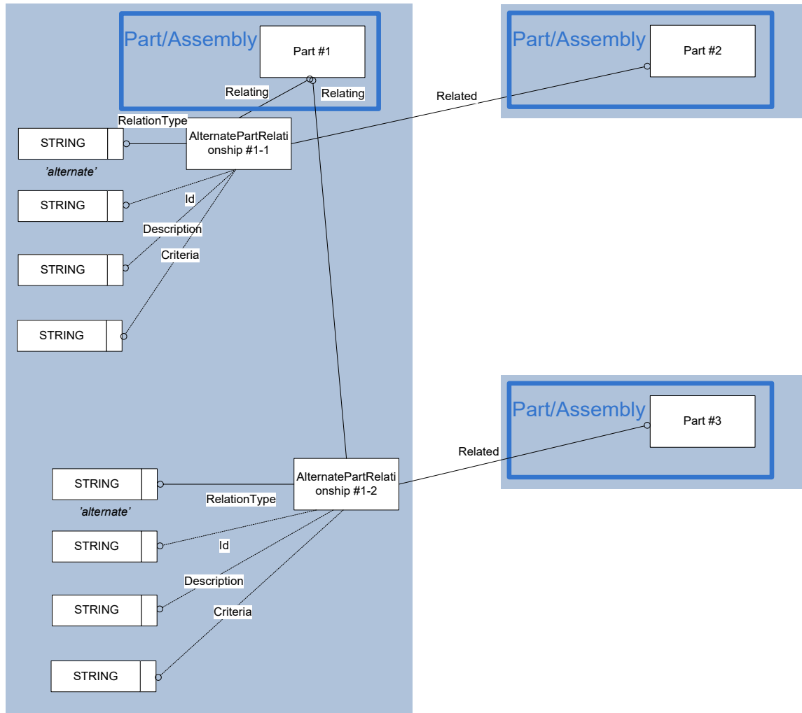
Figure 44: Template "AlternatePartRelationship"
