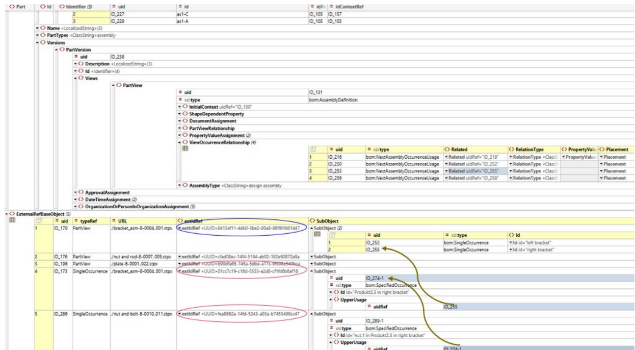
Figure 83: Example of EERs in the parent nested file (as1)
