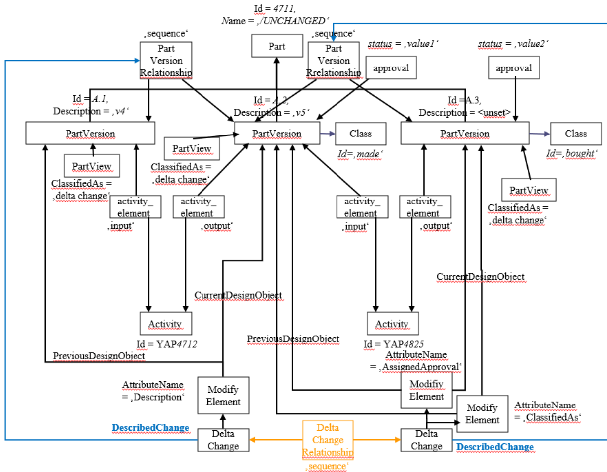
Figure 80: Example of a Delta Exchange for two sequential part changes which order is controlled between two DeltaChanges
