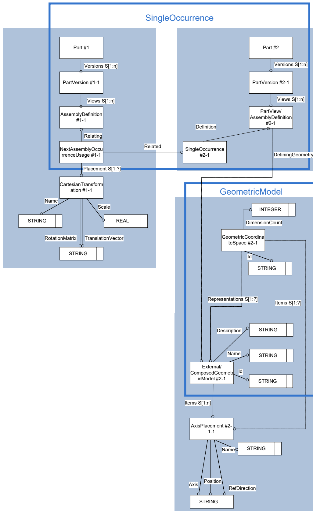
Figure 37: Instantiation example if Part #2 has geometry
