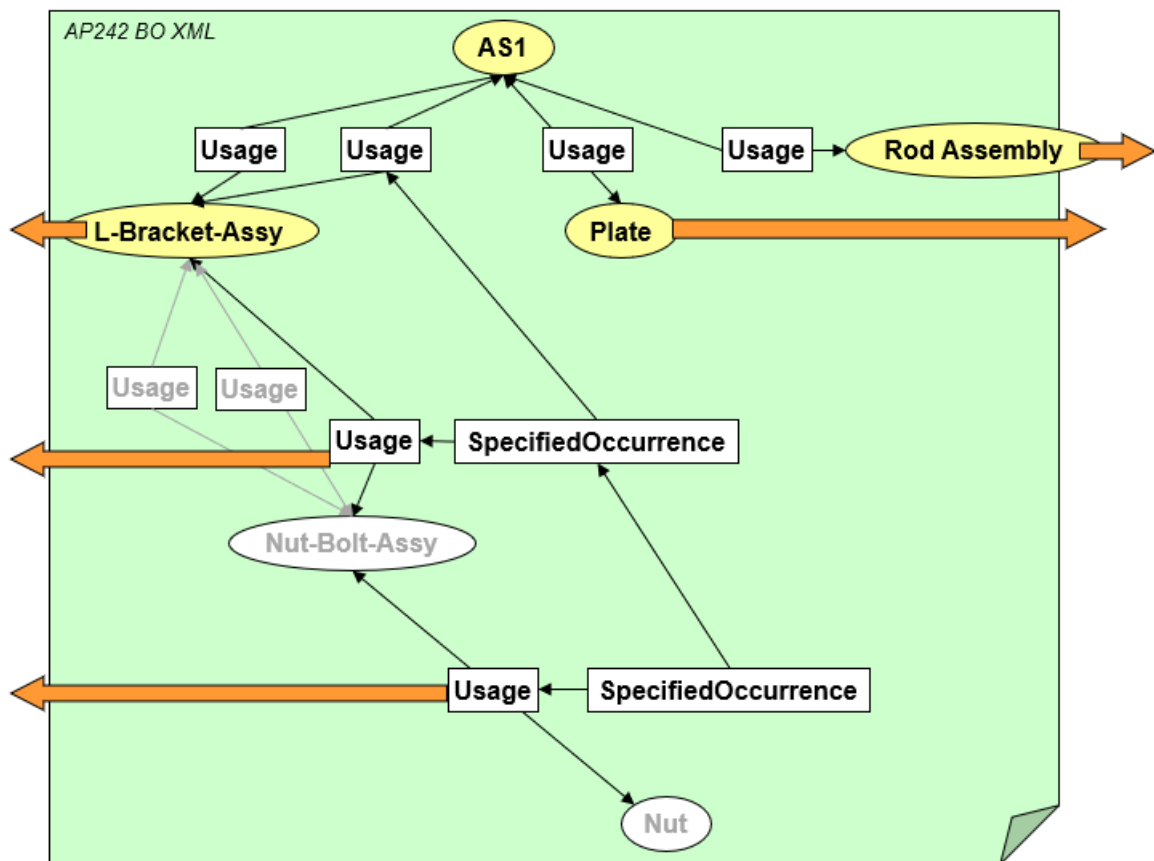
Figure 67: Example for Nested Structure with SpecifiedOccurrences
