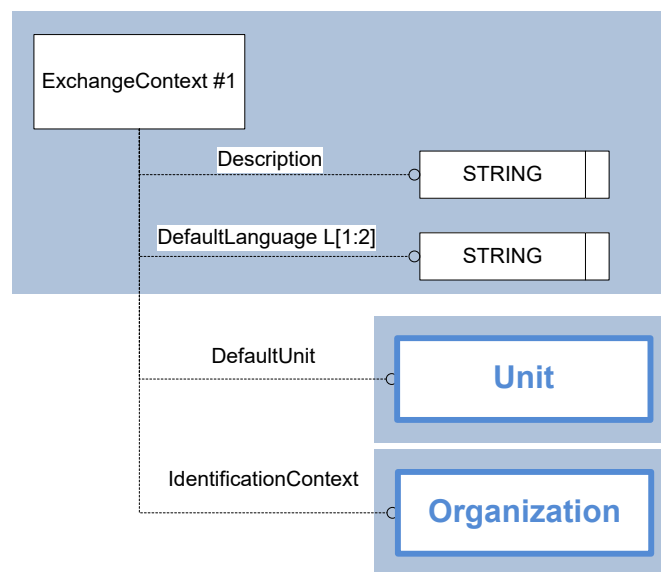
Figure 1: Template “ExchangeContext”
