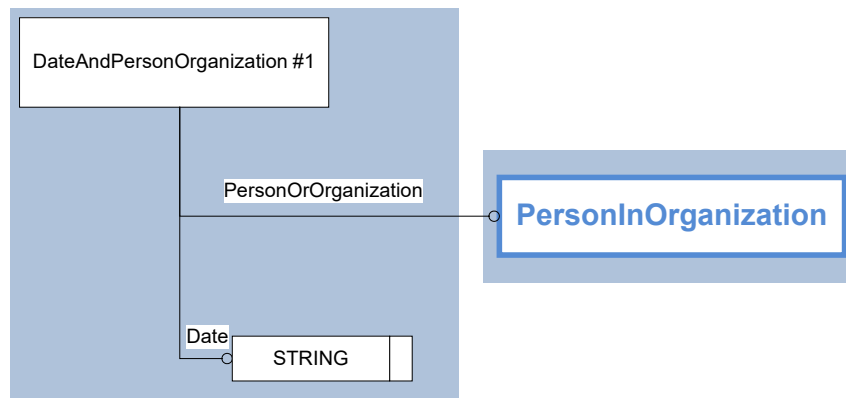
Figure 20: Template “DateAndPersonOrganization”
