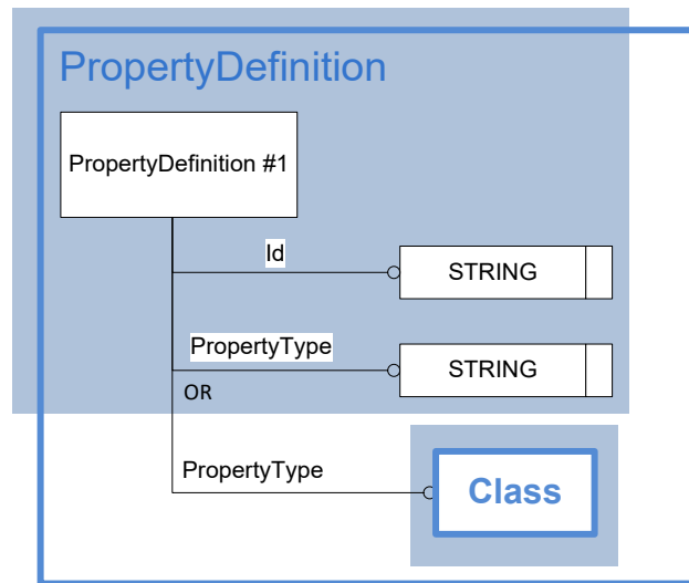
Figure 106: Template "PropertyDefinition"
