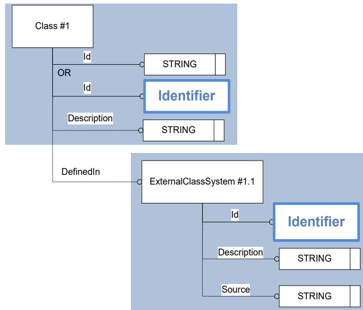
Figure 4: Template "Class"
