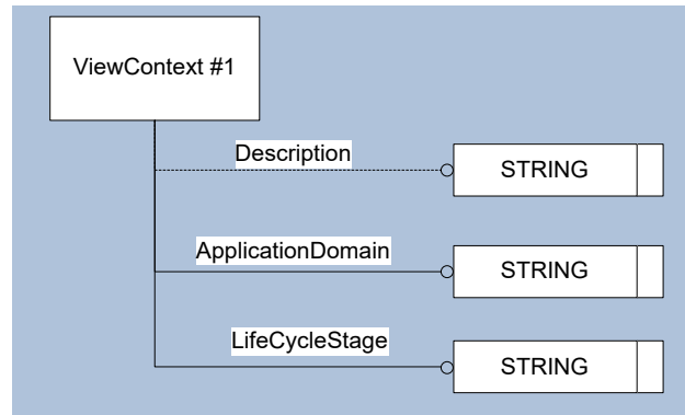
Figure 8: Template "ViewContext"
