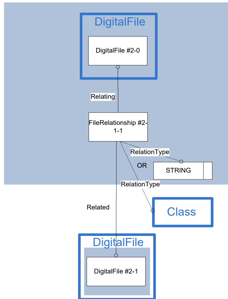
Figure 60: Template “FileRelationship”
