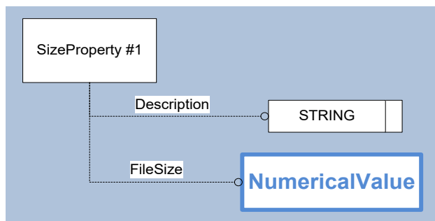
Figure 91: Template “SizeProperty”
