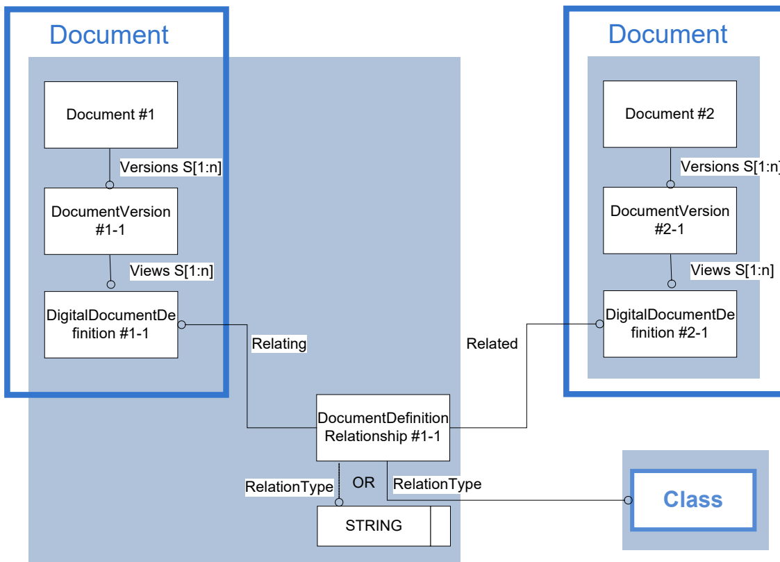
Figure 57: Template “DocumentDefinitionRelationship”
