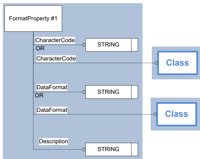
Figure 88: Template “FormatProperty”
