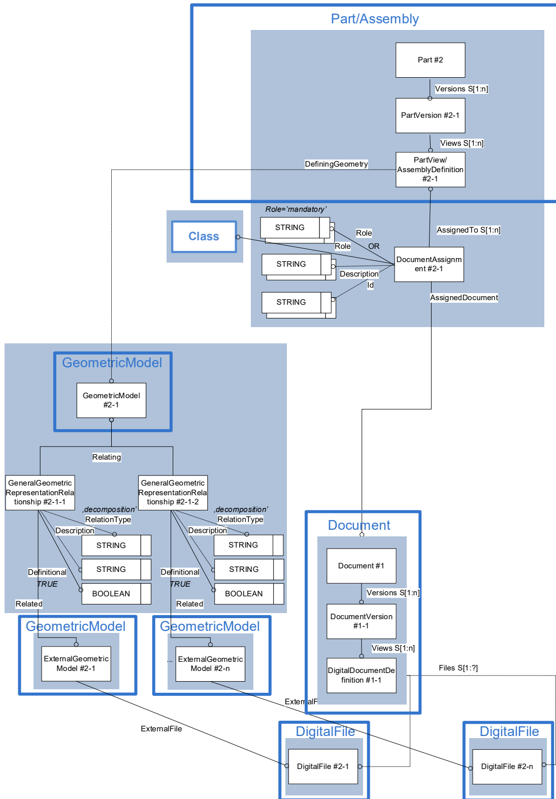
Figure 100: Model splitting in one document for "PDM Representation for DocumentAssignment"
