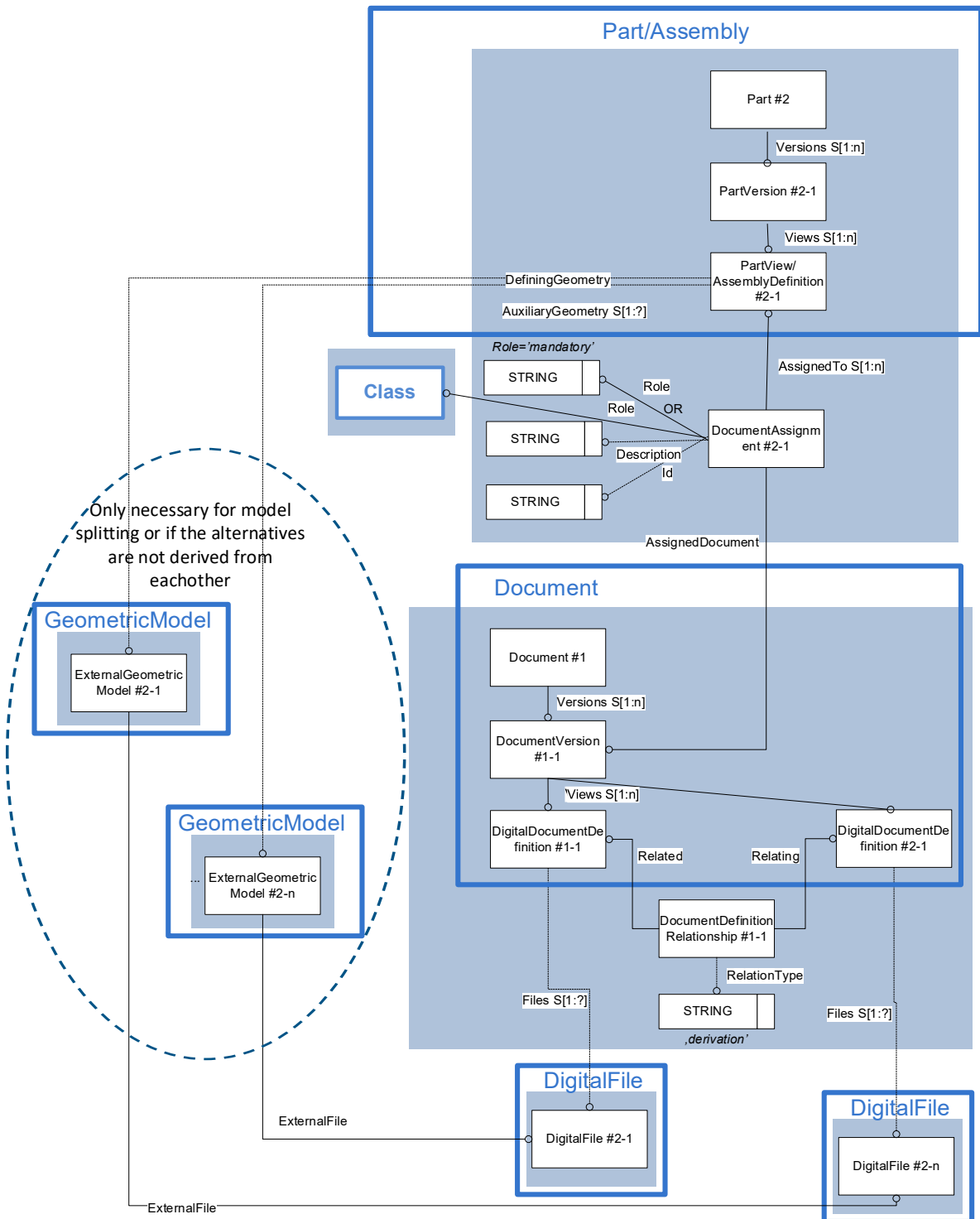
Figure 102: Free alternative files for "PDM Representation for DocumentAssignment"
