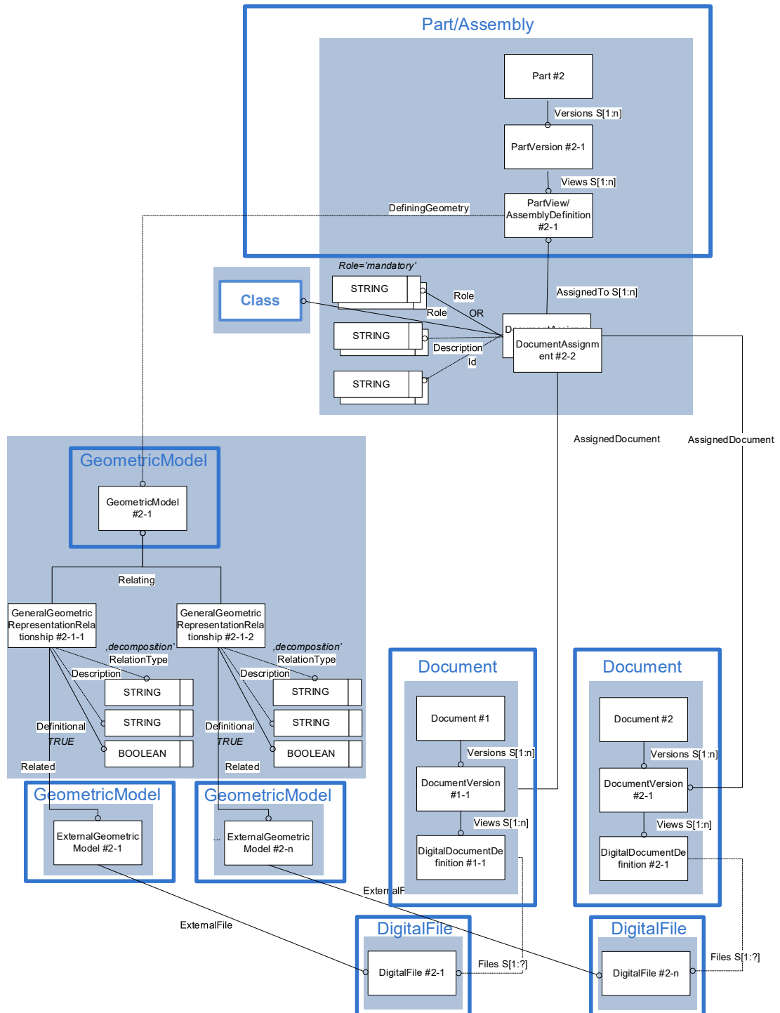
Figure 99: Model splitting in several documents for "PDM Representation for DocumentAssignment"
