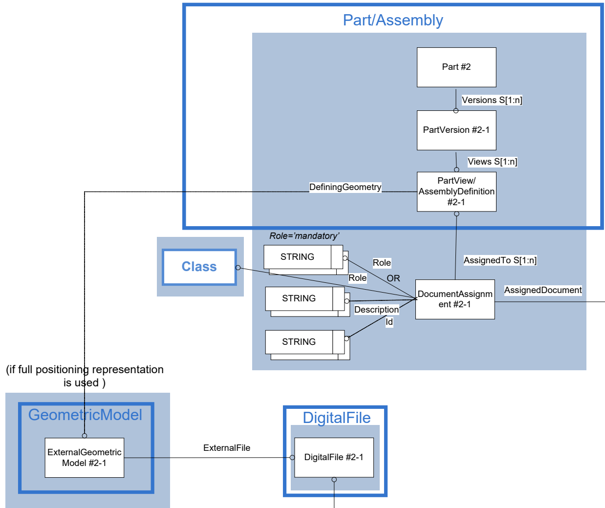
Figure 93: Template "CAx Representation for DocumentAssignment"
