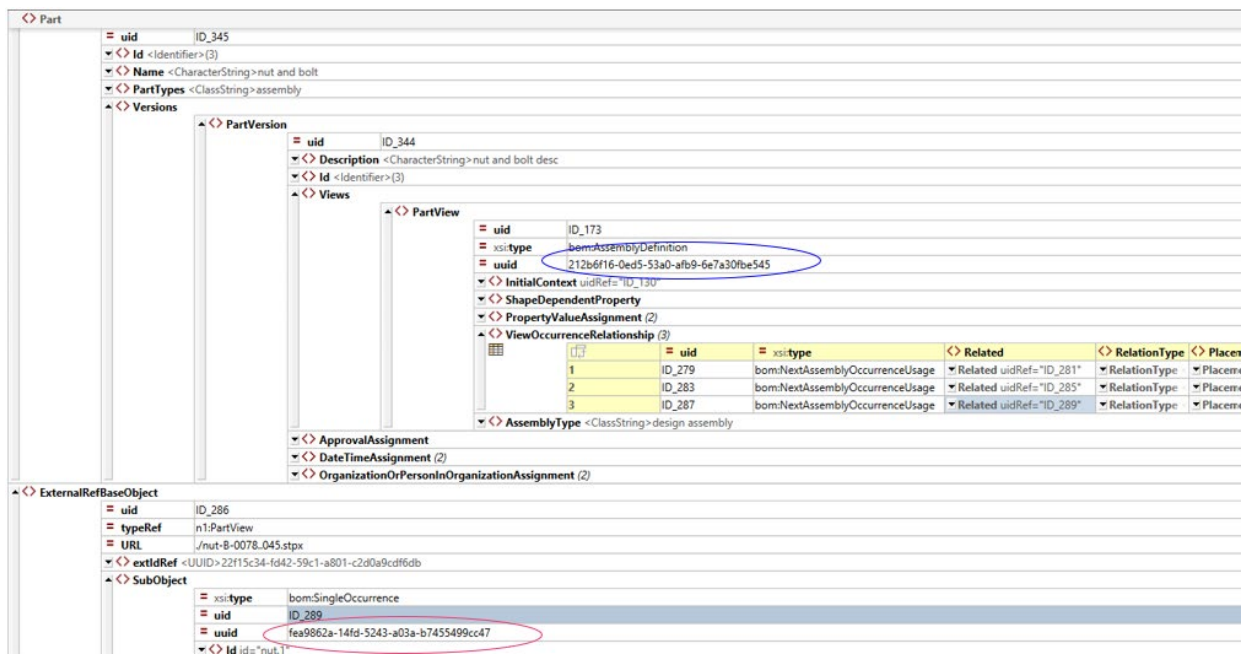
Figure 85: Example of EERs in the child nested file (nut and bolt)
