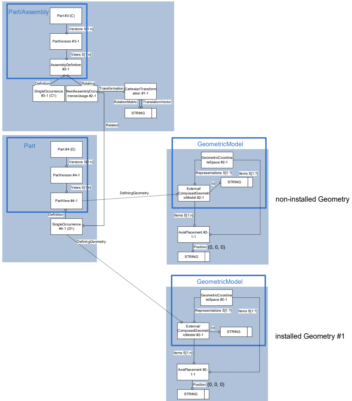
Figure 52: Example of alternative instance shapes based on SingleOccurrences
