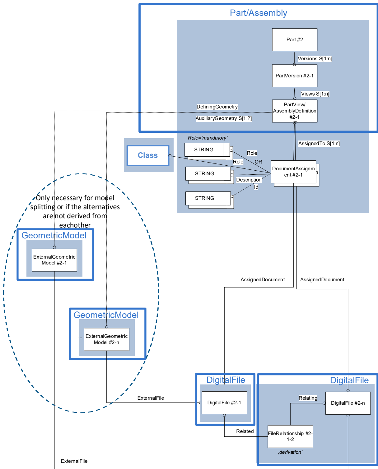
Figure 96: Free alternate models for “CAx Representation for DocumentAssignment”
