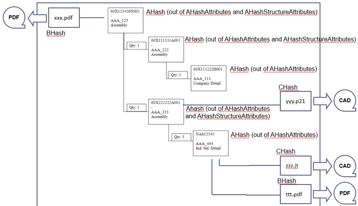
Figure 114: Example of LOTAR Product Structure Validation Properties at the single File, Part and Assembly level
