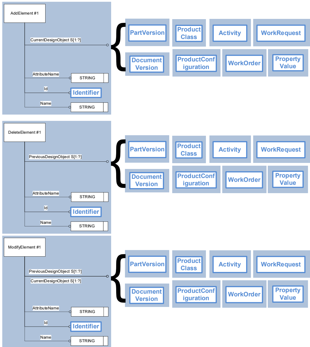
Figure 81: Template "DeltaChangeActivity"
