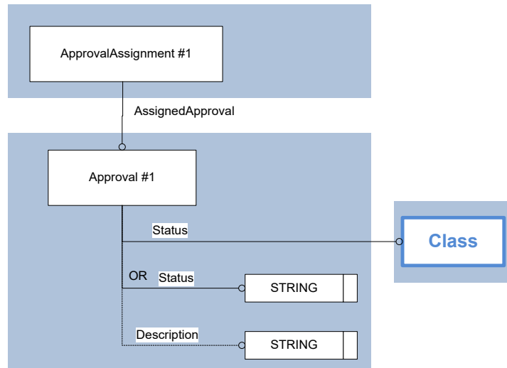
Figure 17: Template "Approval"
