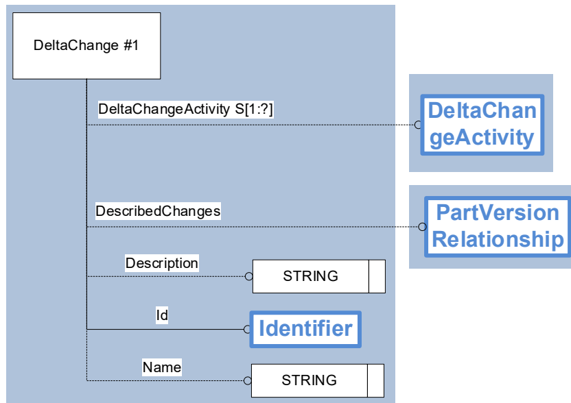
Figure 79: Template "DeltaChange"
