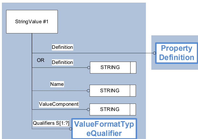
Figure 10: Template “StringValue”
