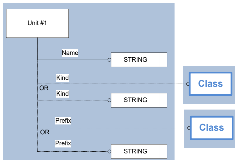
Figure 3: Template “Unit”
