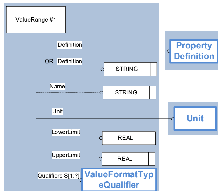
Figure 11: Template "ValueRange"
