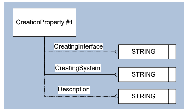
Figure 90: Template “CreationProperty”
