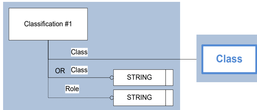
Figure 5: Template "Classification"
