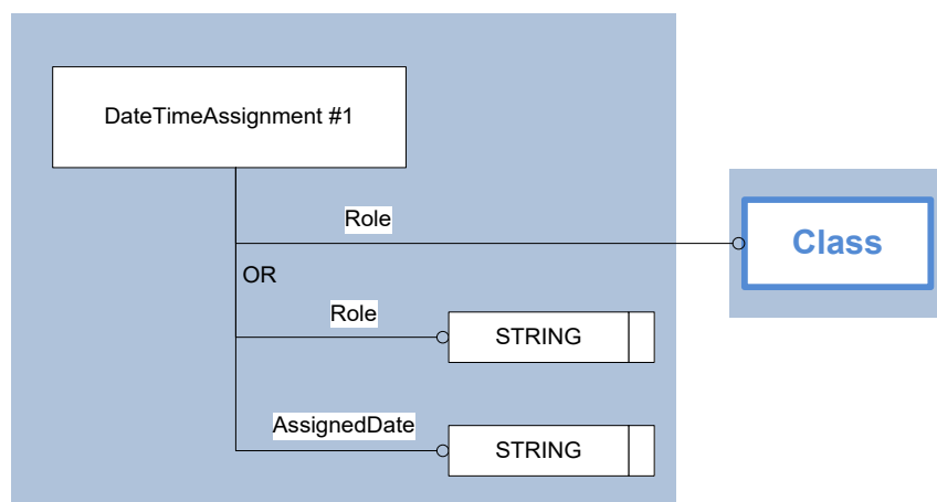
Figure 16: Template “DateTime”
