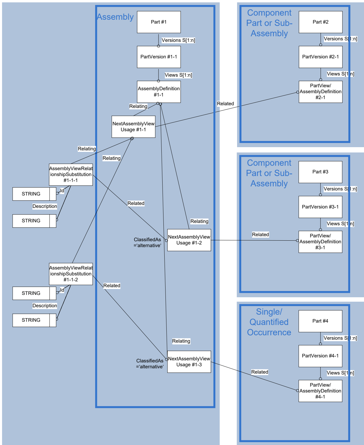
Figure 47: Template "AssemblyViewRelationshipSubstitution"
