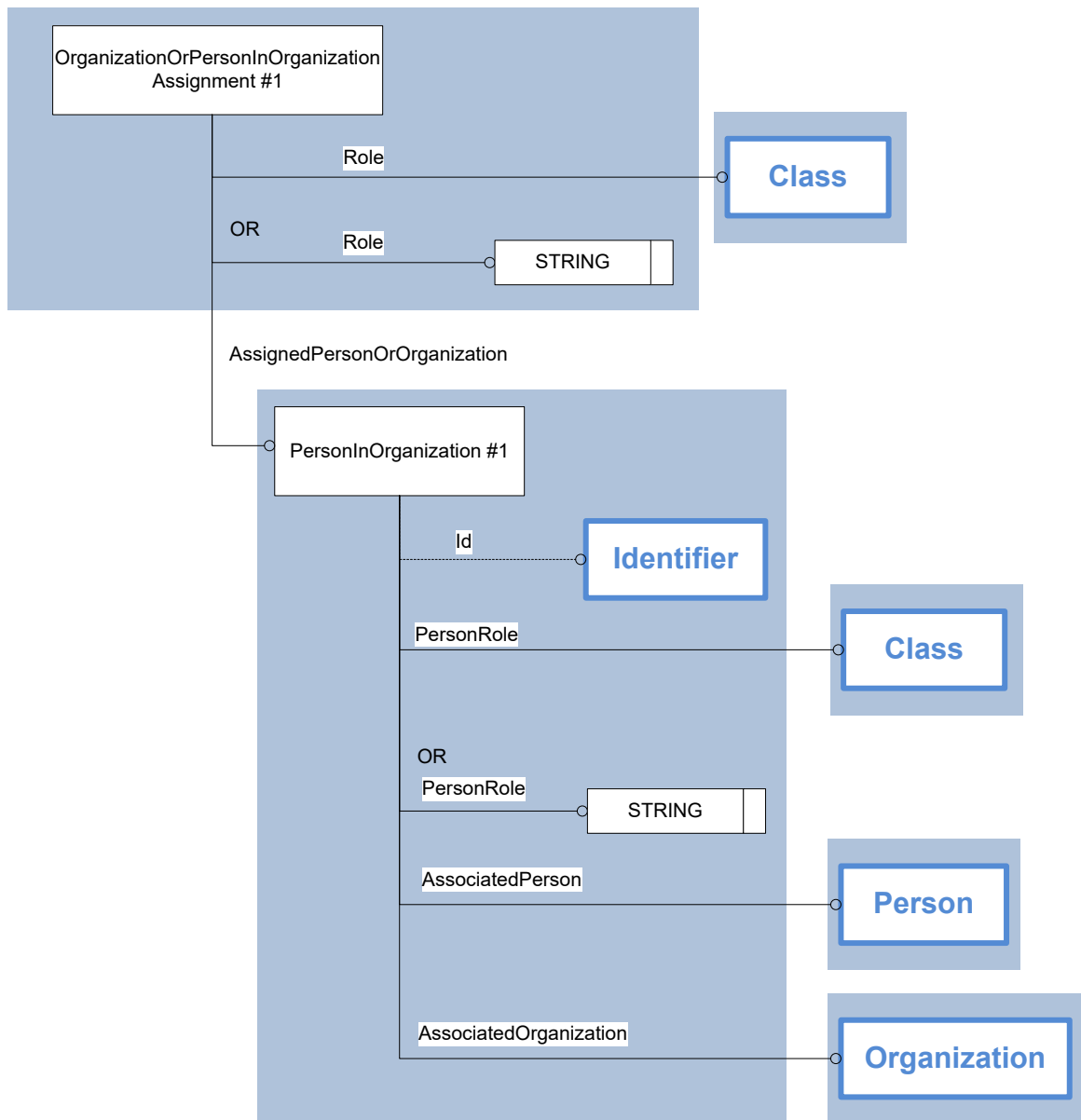
Figure 19: Template “PersonInOrganization”
