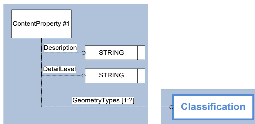
Figure 89: Template “ContentProperty”
