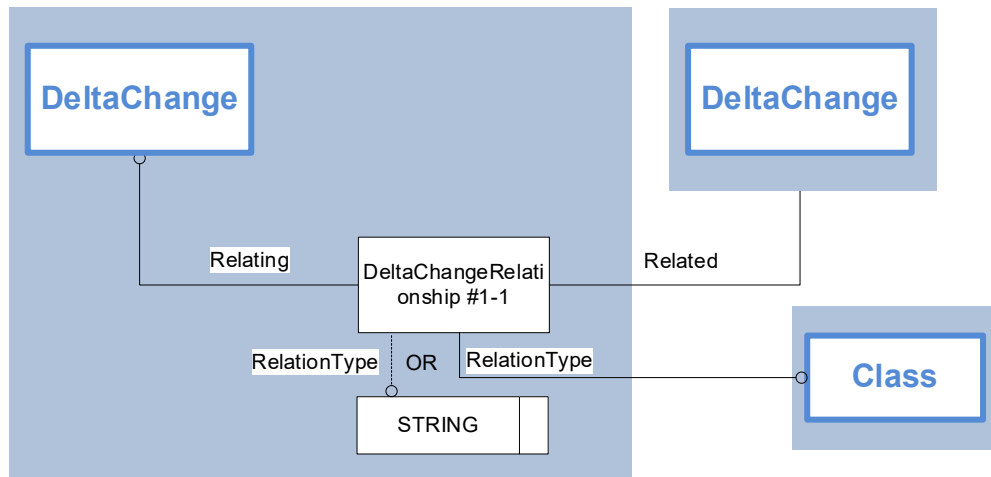
Figure 82: Template "DeltaChangeRelationship"
