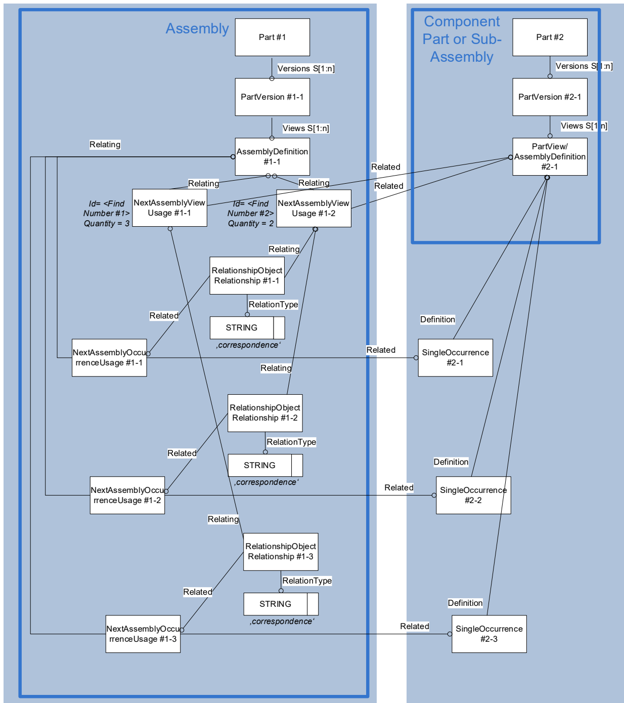
Figure 55: Template "RelationshipObjectRelationship"
