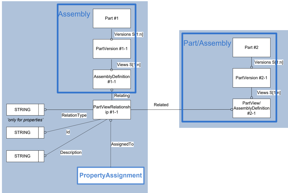
Figure 42: Template "PartViewRelationship" for properties
