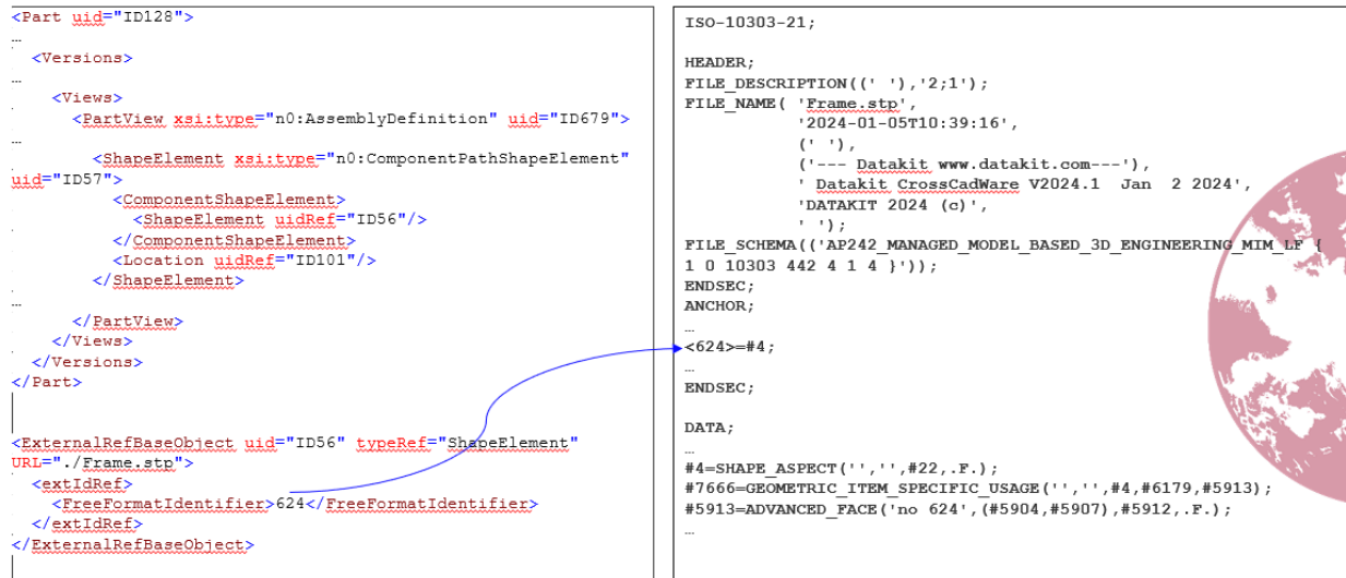
Figure 86: Example of an EER to an anchor element within a Part 21 geometry file
