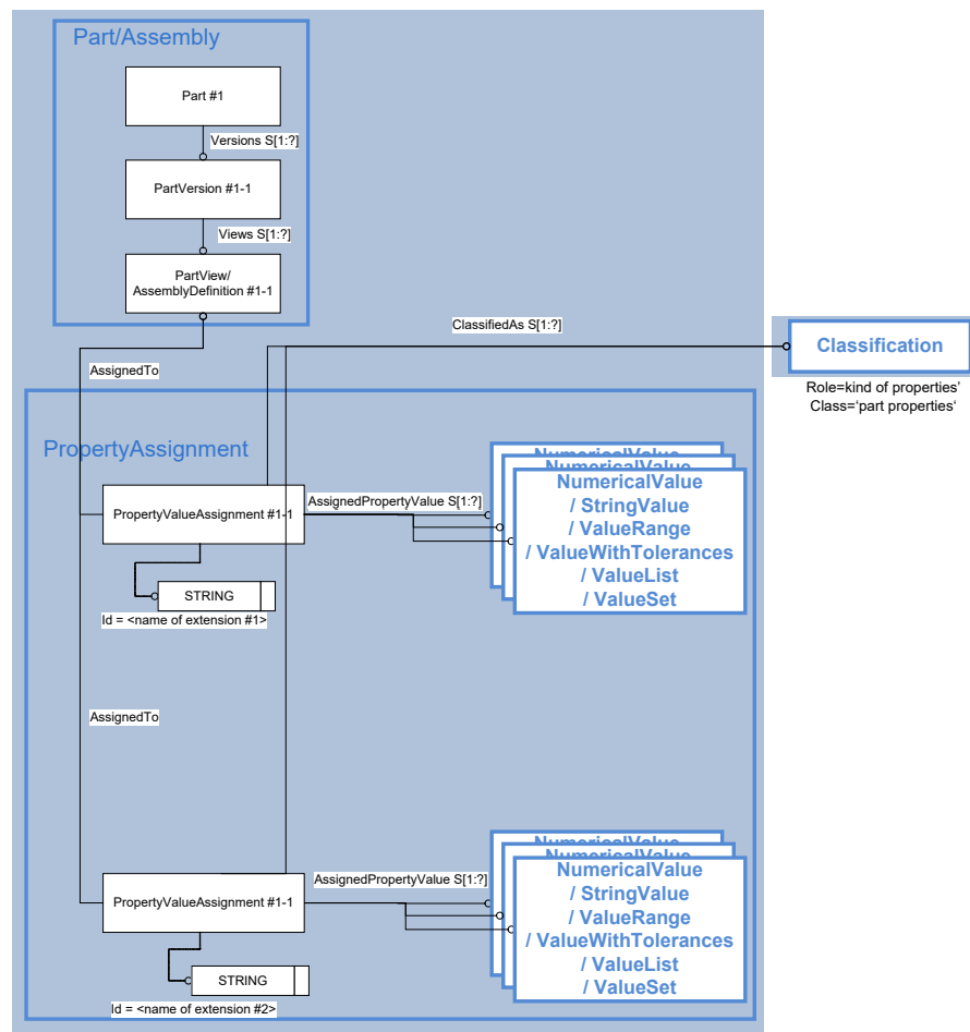
Figure 119: Example of property groups on a Part having properties on the PartView.
