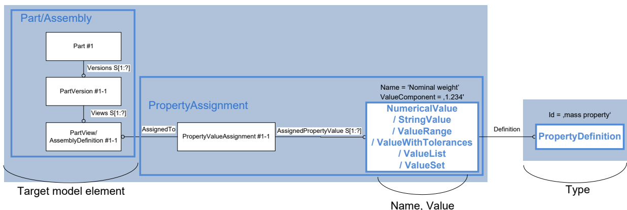
Figure 107: User defined attribute at the part/assembly level
