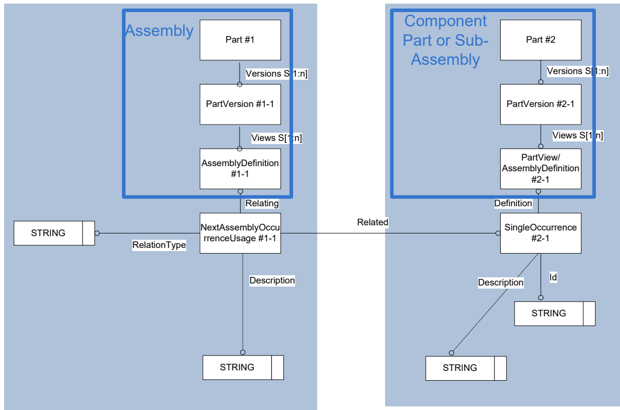
Figure 30: Template "SingleOccurrence"
