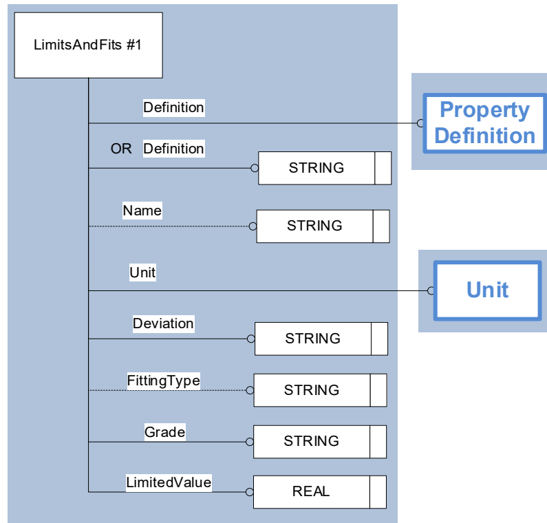
Figure 13: Template “LimitsAndFits”
