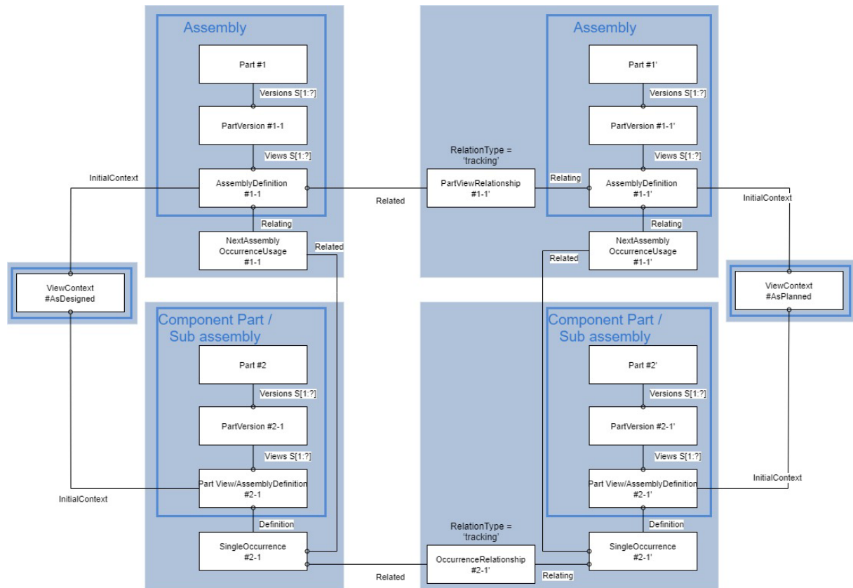
Figure 121: Representation of tracking relationship
