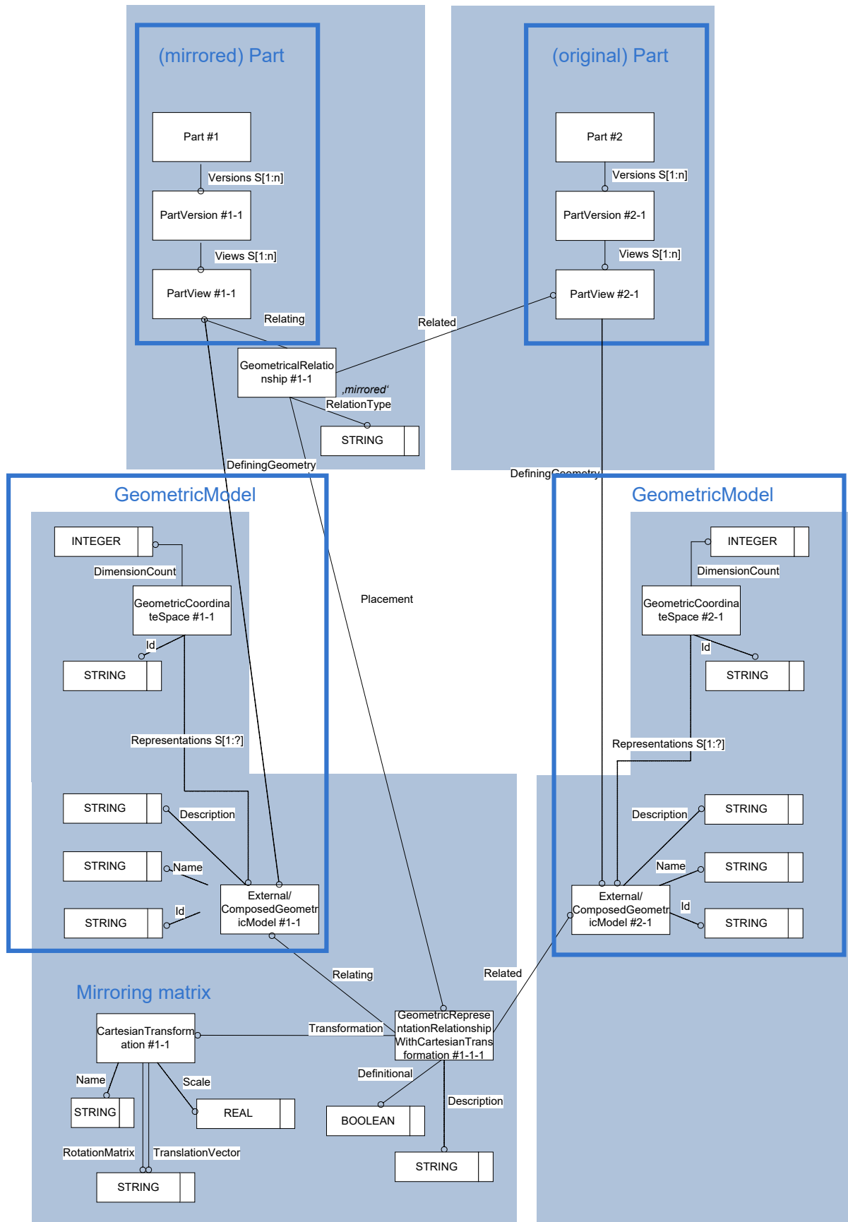
Figure 50: Template "Full Mirroring Positioning Representation"
