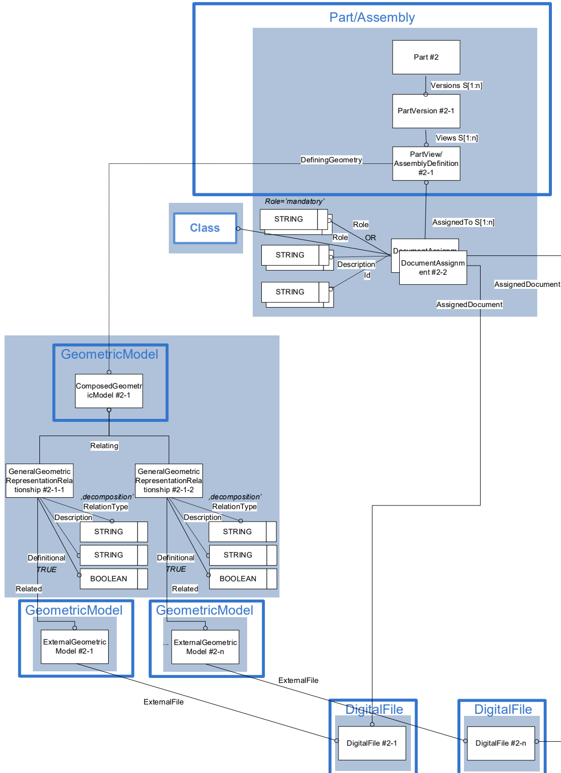
Figure 95: Model splitting for "CAx Representation for DocumentAssignment"
