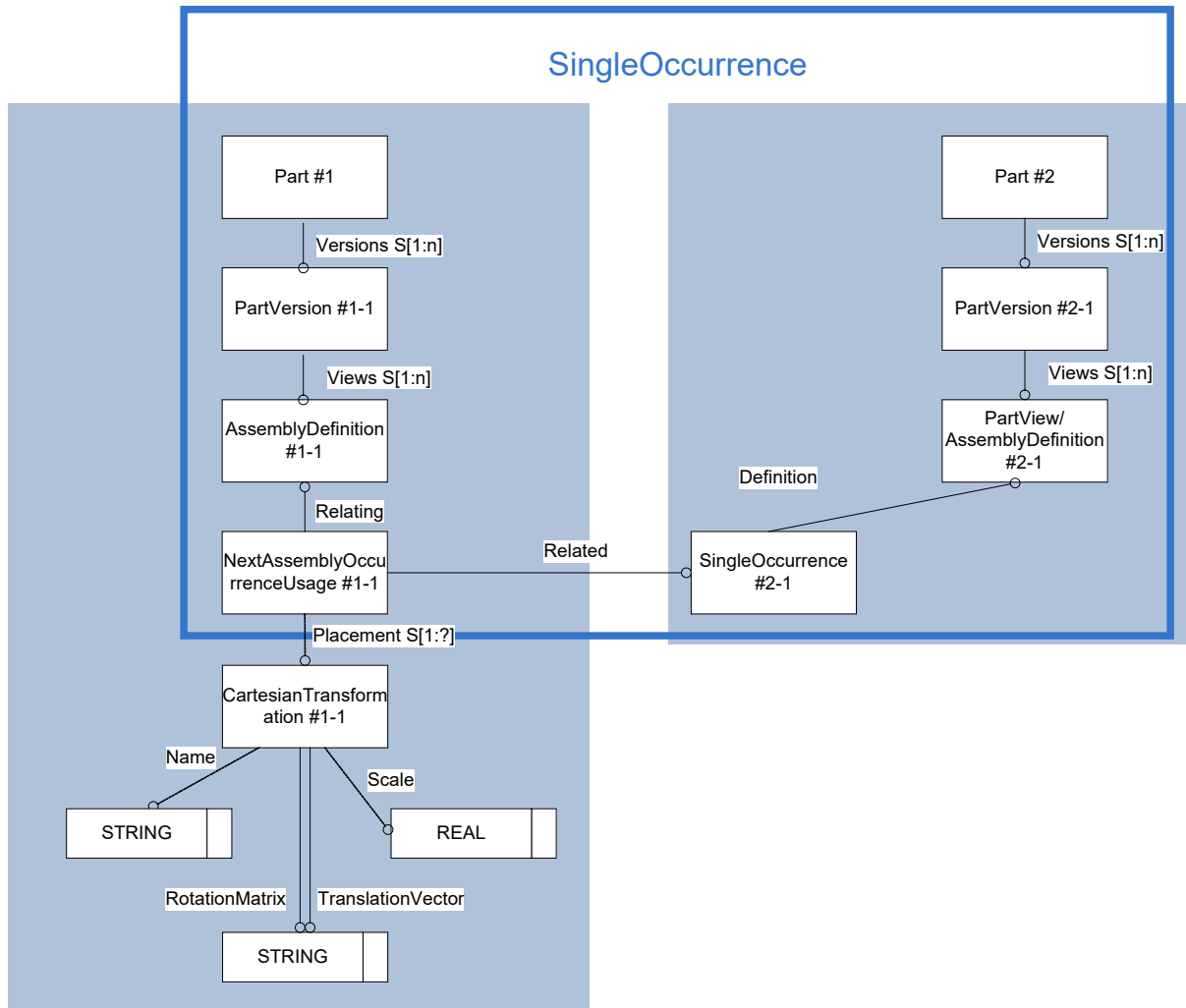
Figure 36: Template "Simplified Positioning Representation"
