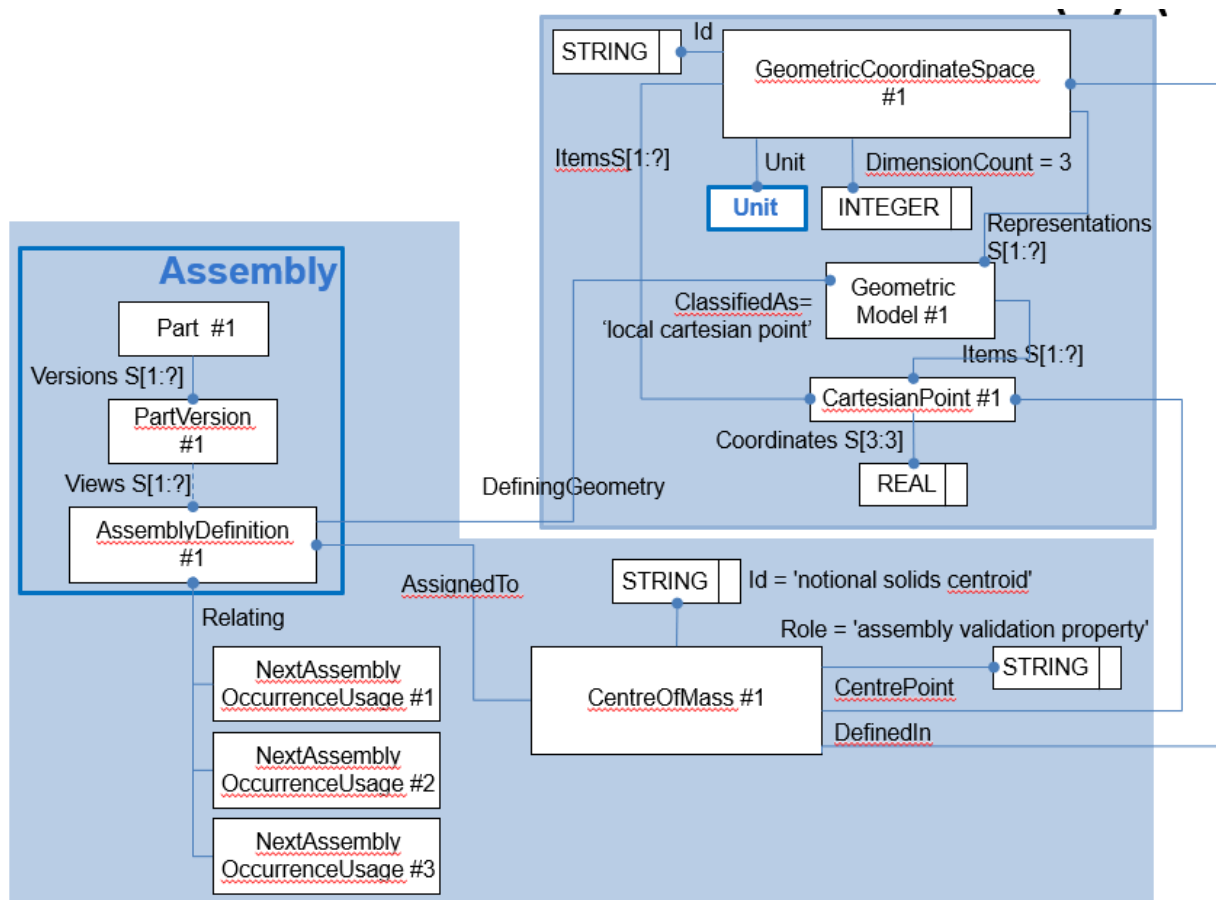
Figure 113: Instantiation of AVP 'notional solids centroid'
