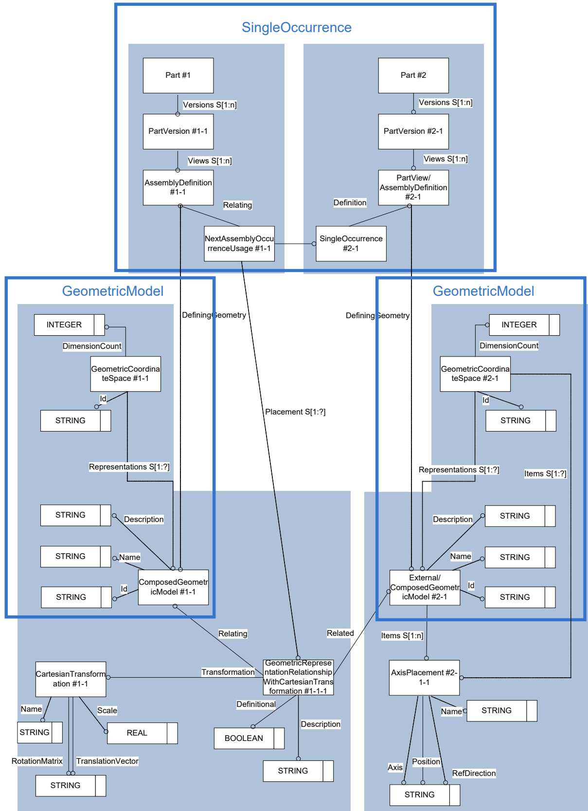
Figure 39: Full Positioning Representation with Explicit Transformation
