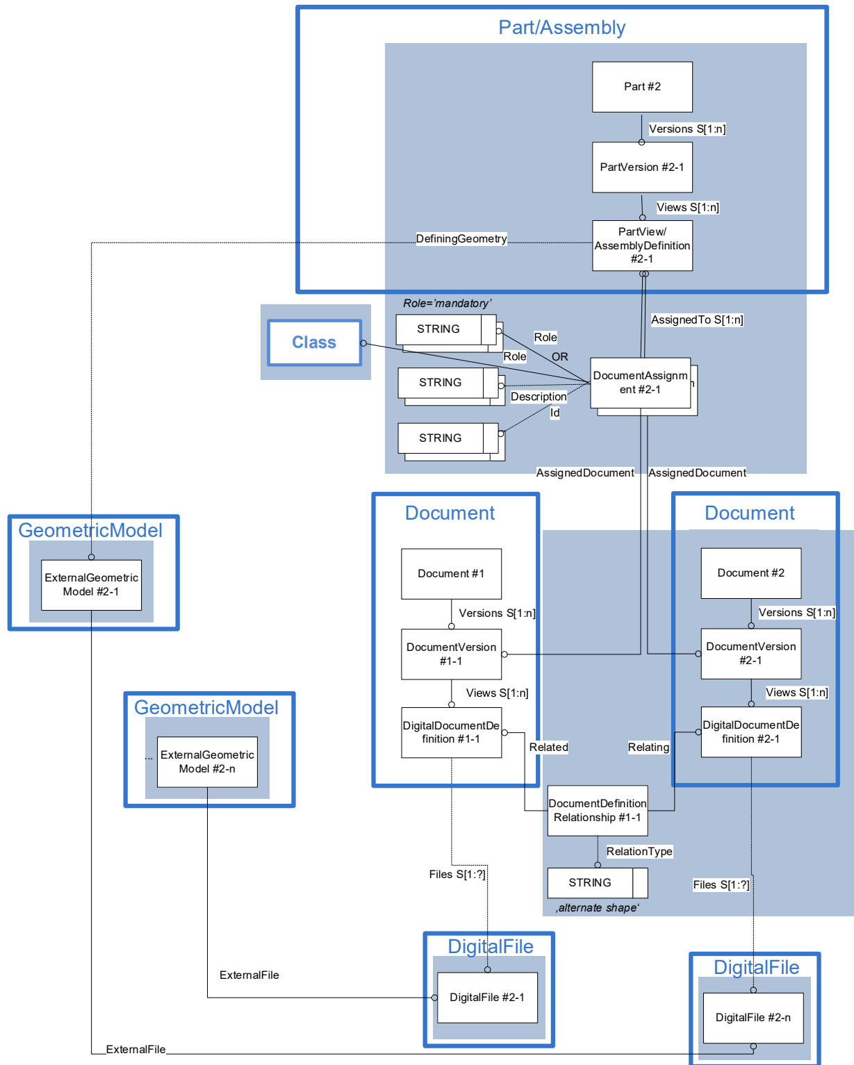
Figure 103: Forced Alternative documents for "PDM Representation for DocumentAssignment"
