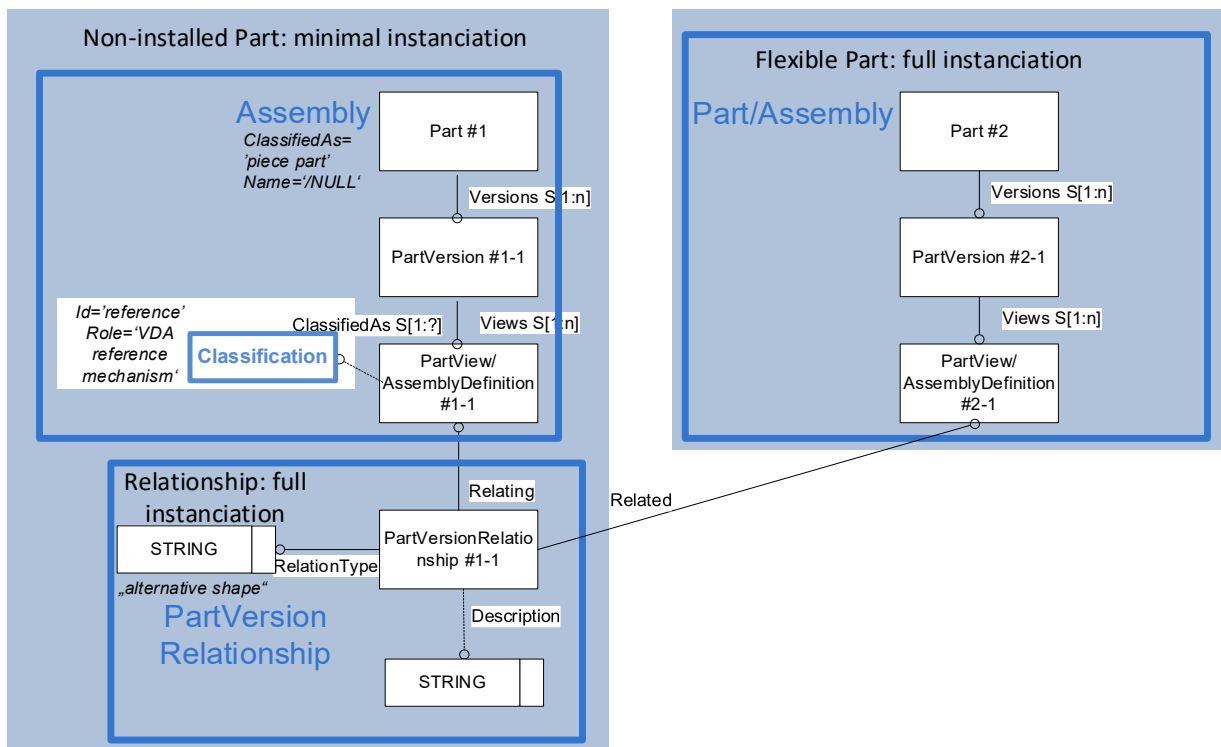
Figure 68: Special handling of additional 'Related' Parts after archiving/releasing the 'Relating' Part (here example of an additional shape as Flexible Part)
