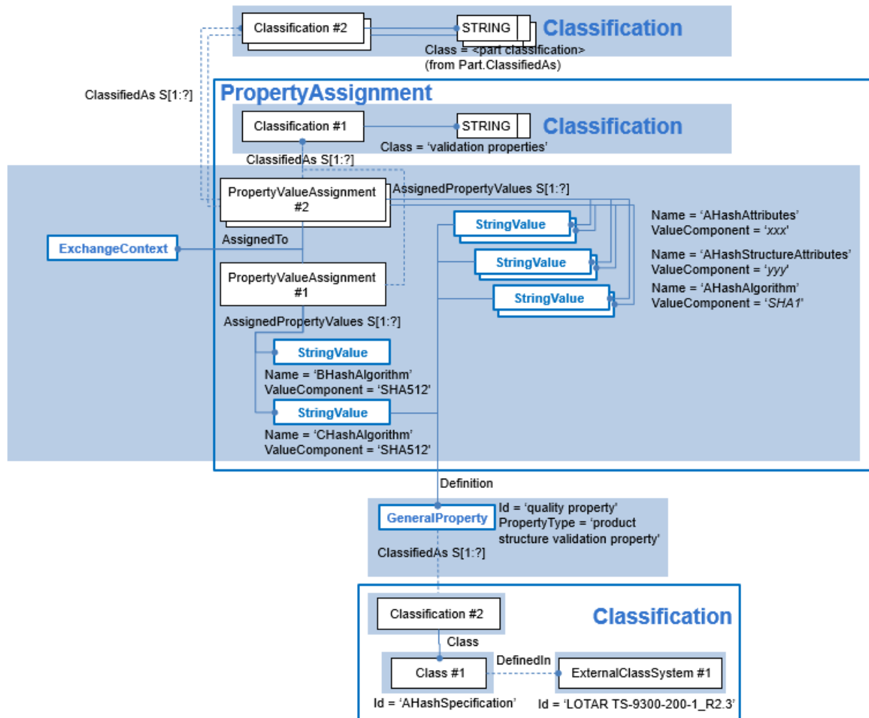
Figure 117: Template "AHash[Structure]Attributes and A/B/CHashAlgorithm on ExchangeContext"
