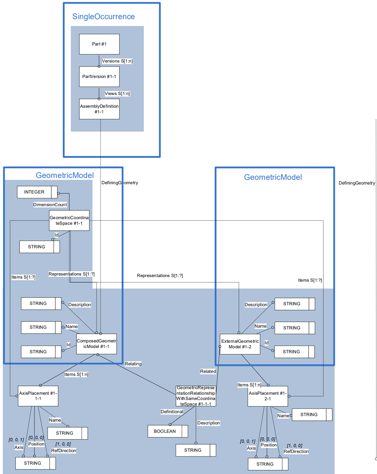
Figure 94: Template "CAx Representation for Geometry at Assembly Level"
