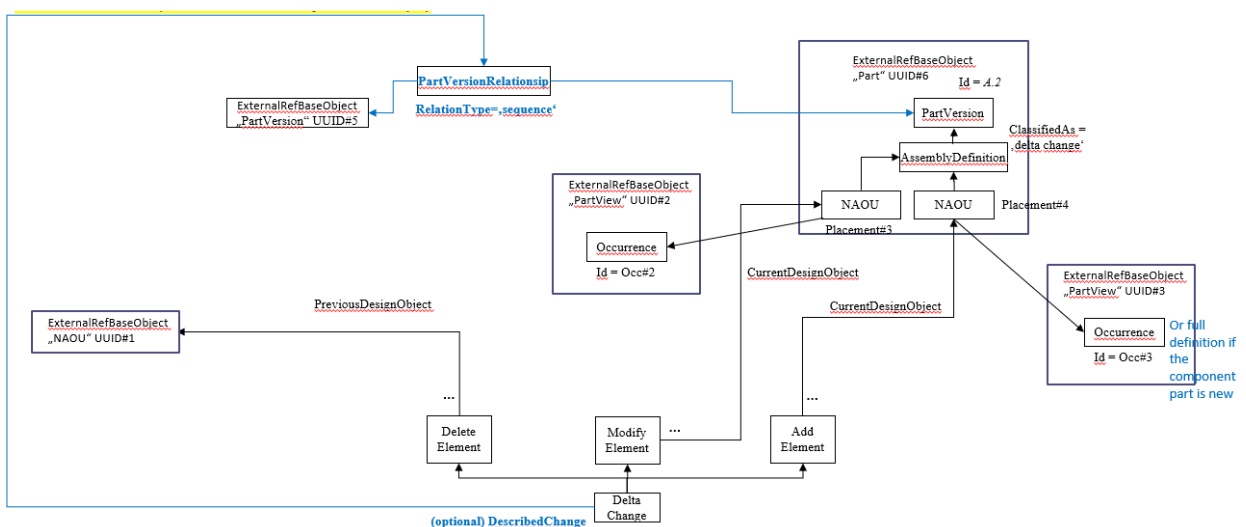
Figure 76: Example of a Delta Exchange on an assembly part with one component deleted, one added and one modified (using EER Mechanism)
