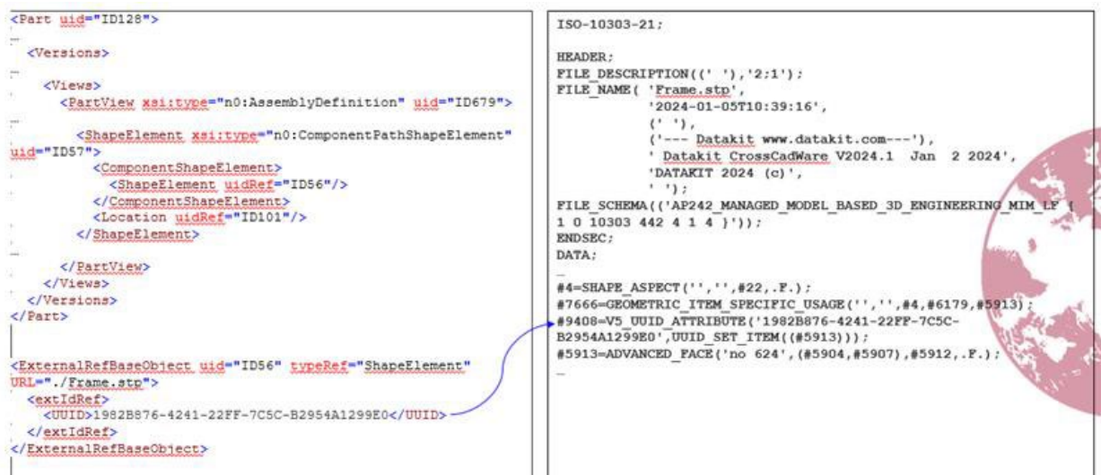
Figure 87: Example of an EER to a Data Section element within a Part 21 geometry file
