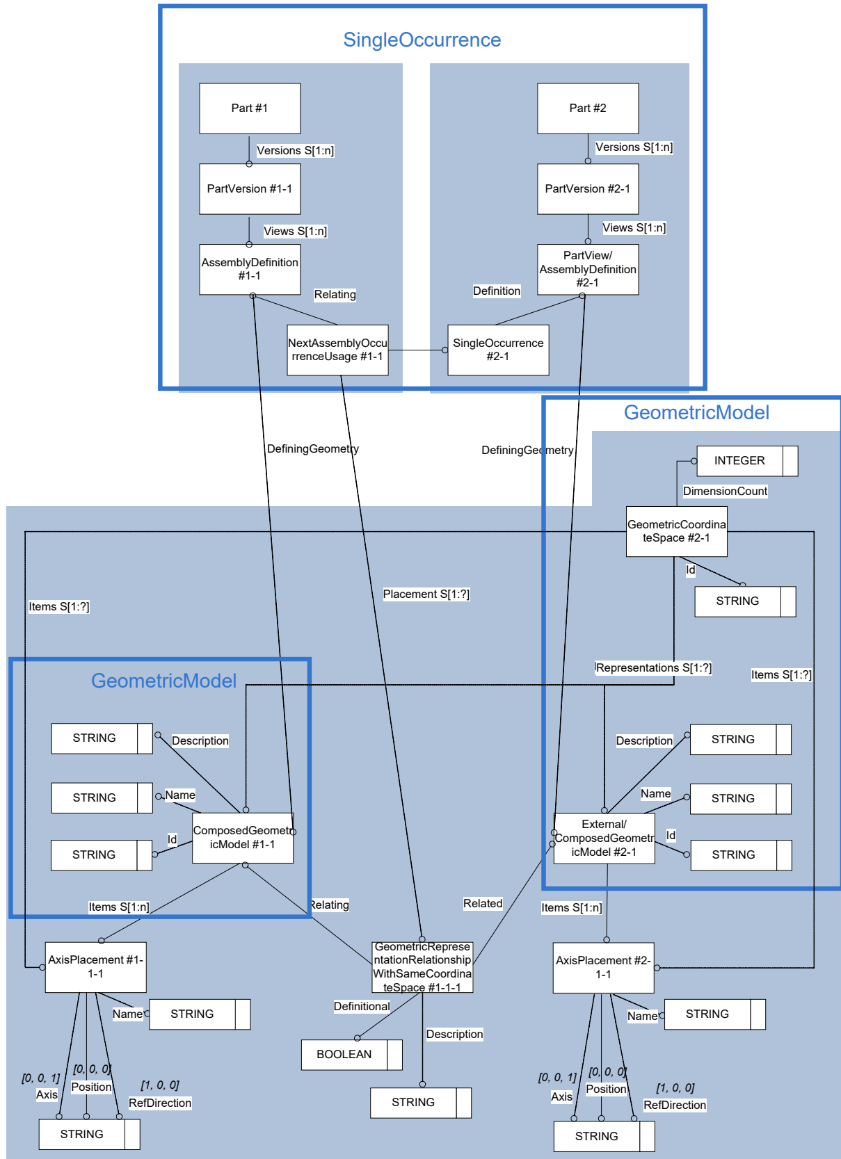
Figure 40: Full Positioning Representation with Same Coordinate Space
