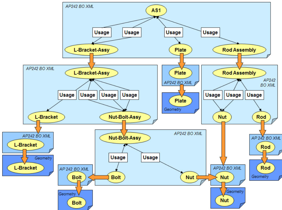
Figure 62: Example for Nested Structure with additional part-level XML files
