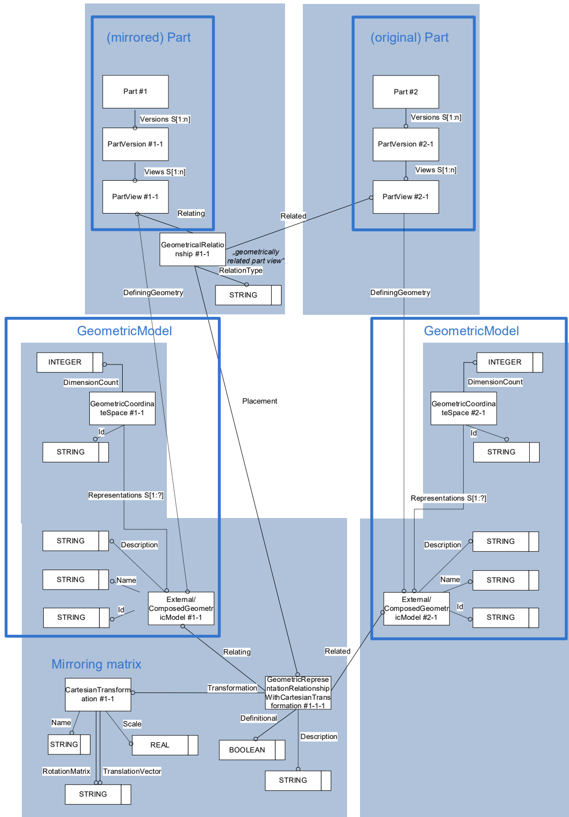
Figure 49: Template "Simplified Mirroring Positioning Representation"
