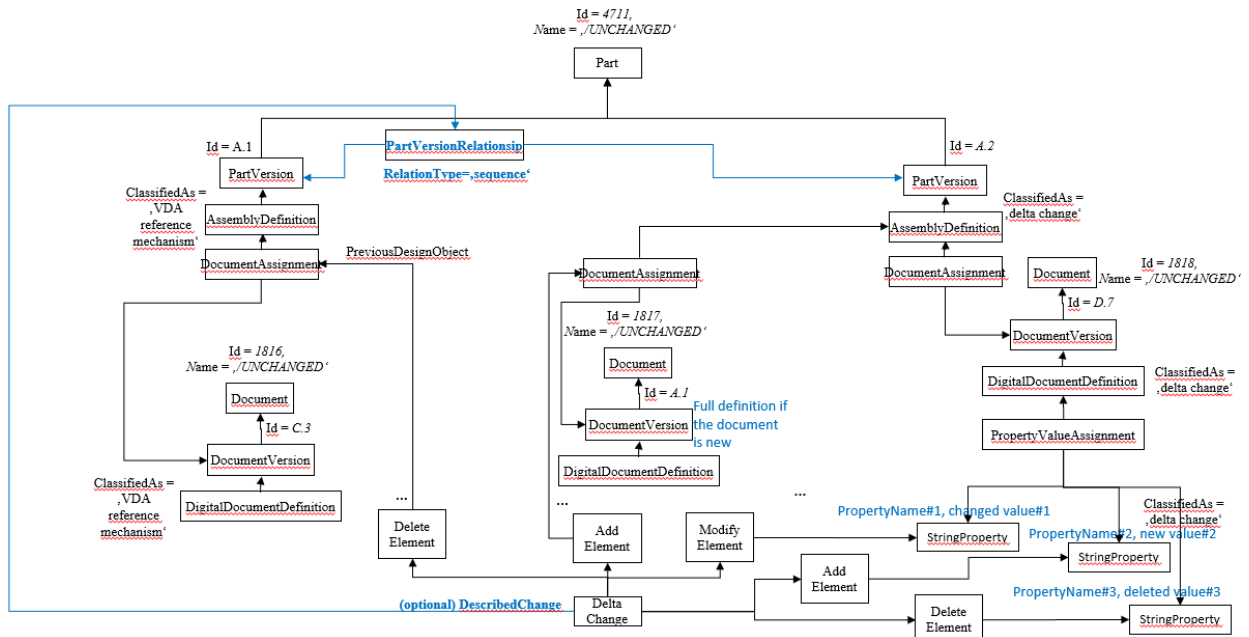
Figure 75: Example of Delta Exchange of a new part version with one document deleted, one added and one modified (using Reference Mechanism)
