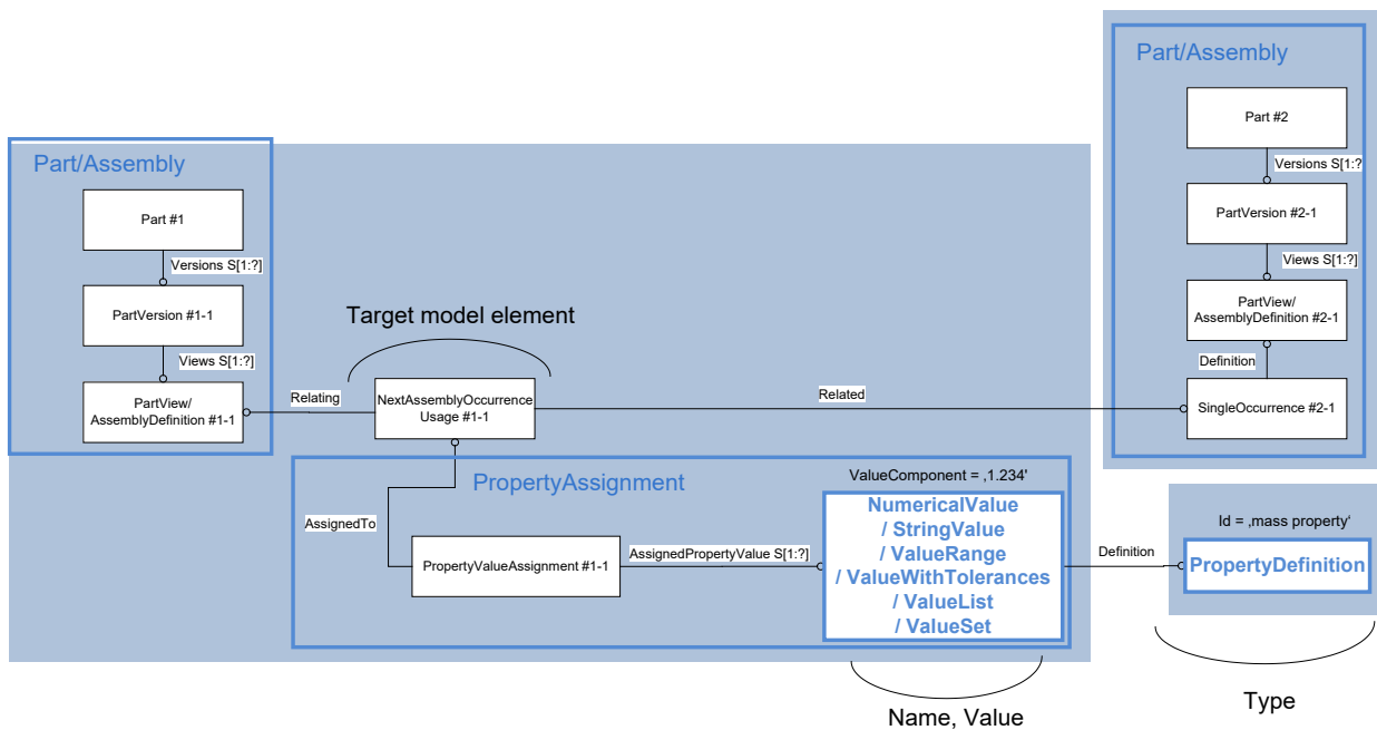
Figure 108: User defined attribute for a simple component instance in an assembly
