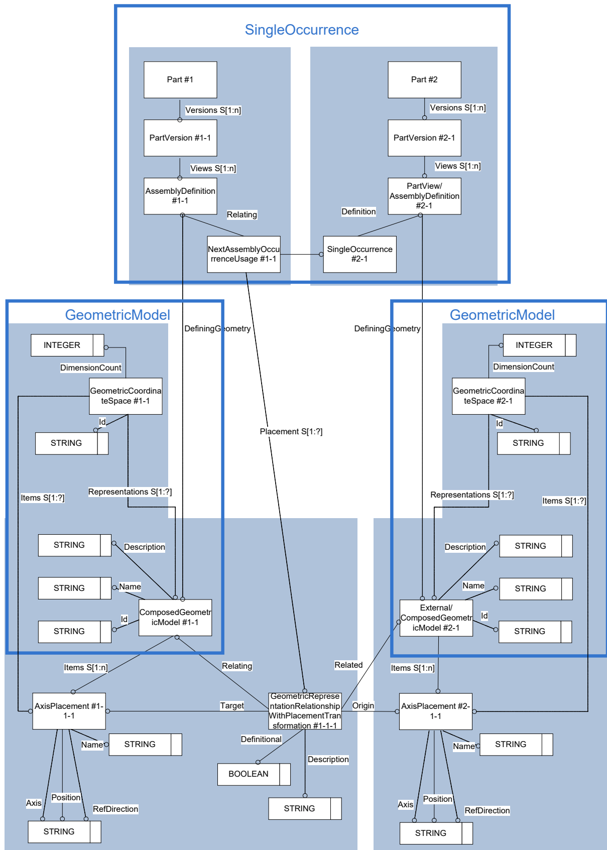
Figure 38: Full Positioning Representation with Implicit Transformation
