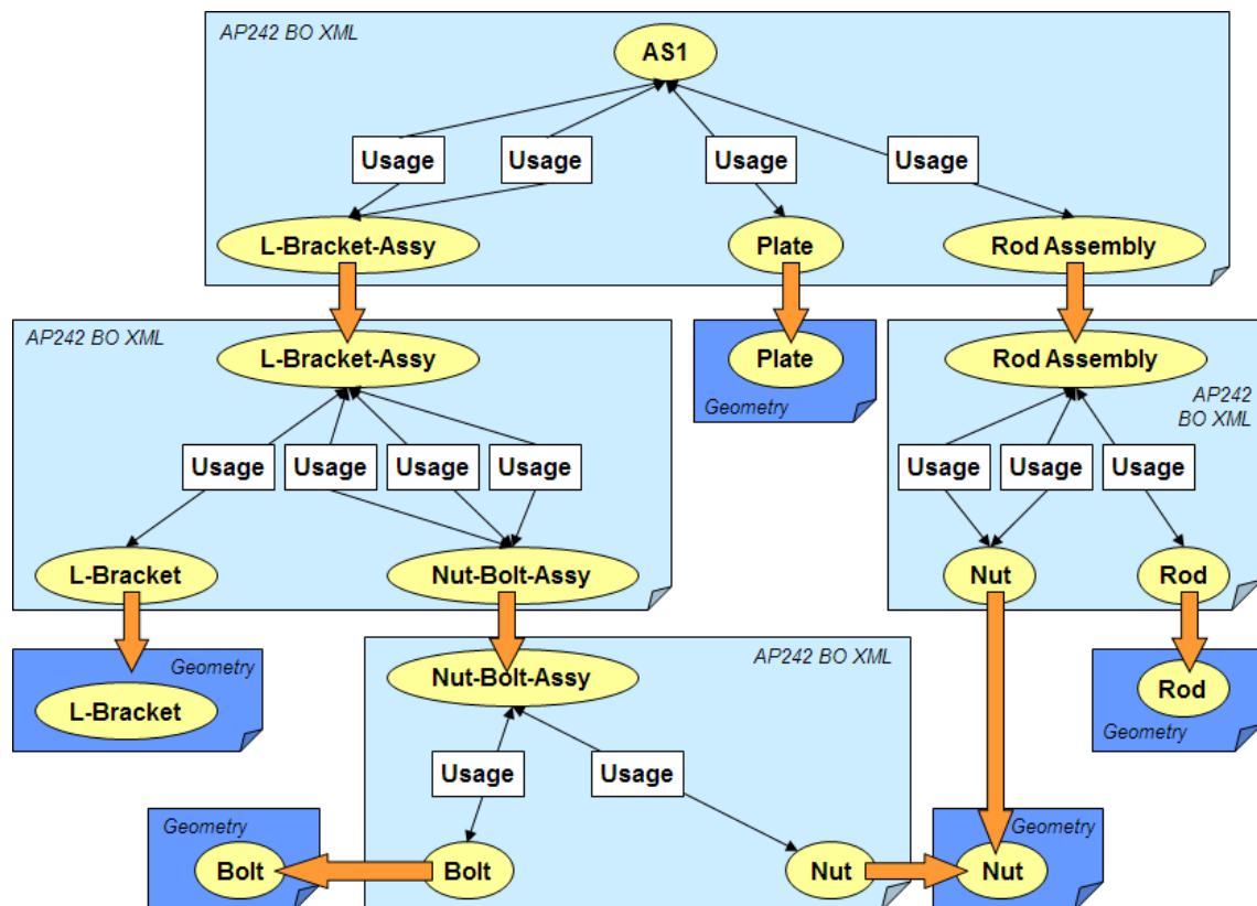
Figure 61: Example for not recommended Nested Structure
