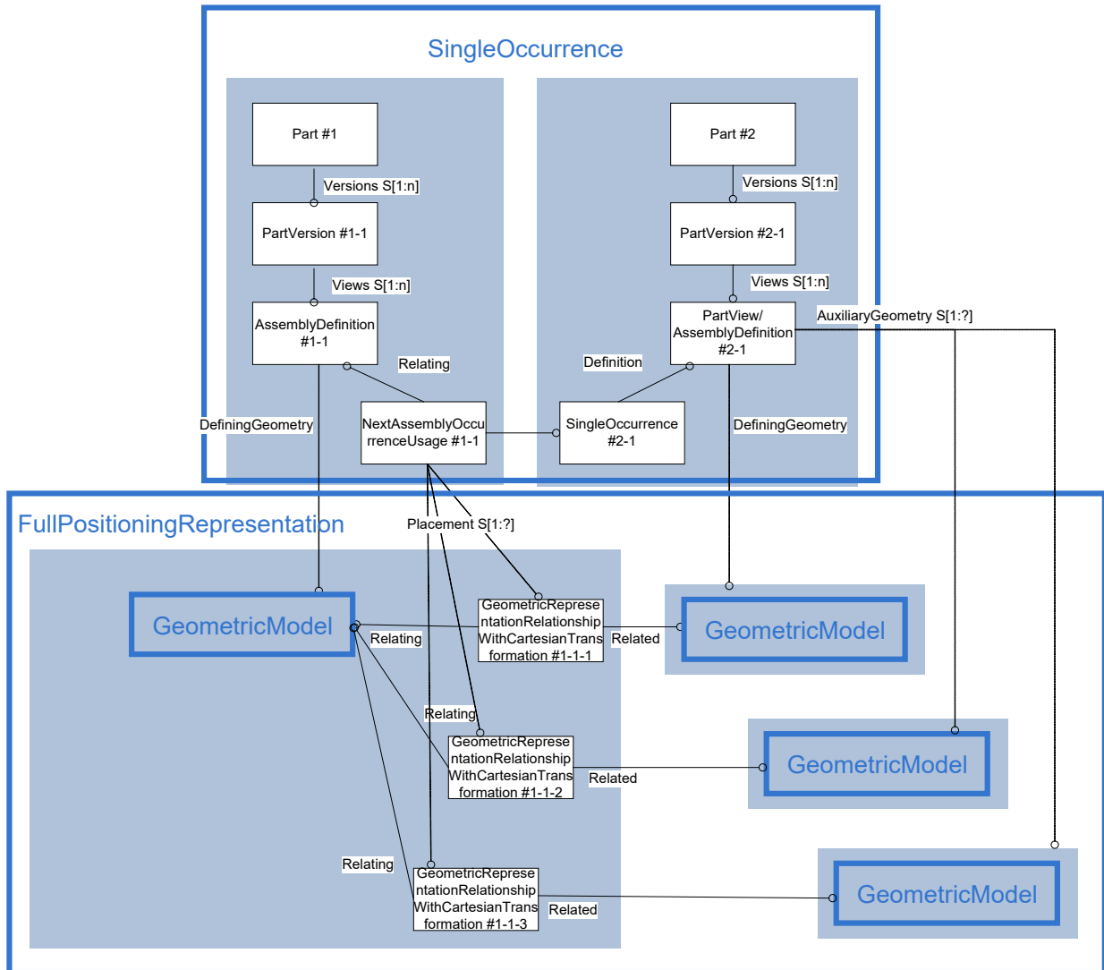
Figure 31: Cross-reference of Defining/AuxiliaryGeometry and NextAssemblyOccurrenceUsage.Placement
