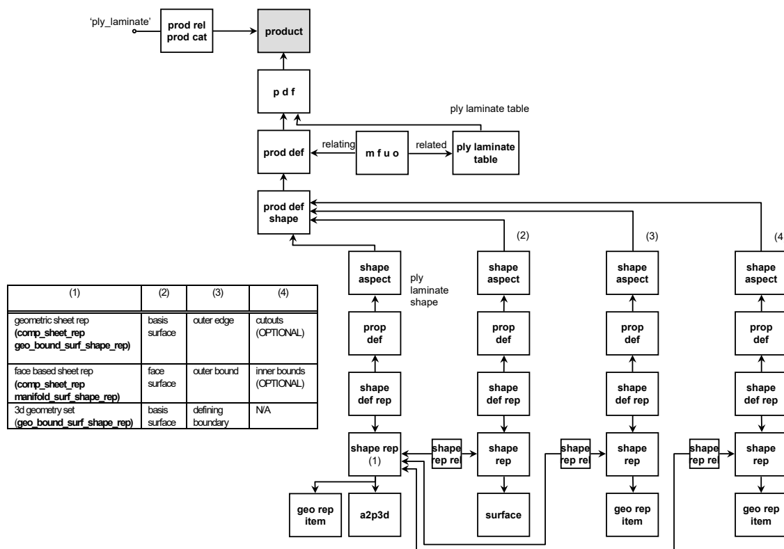
Figure 28: Ply Laminate
