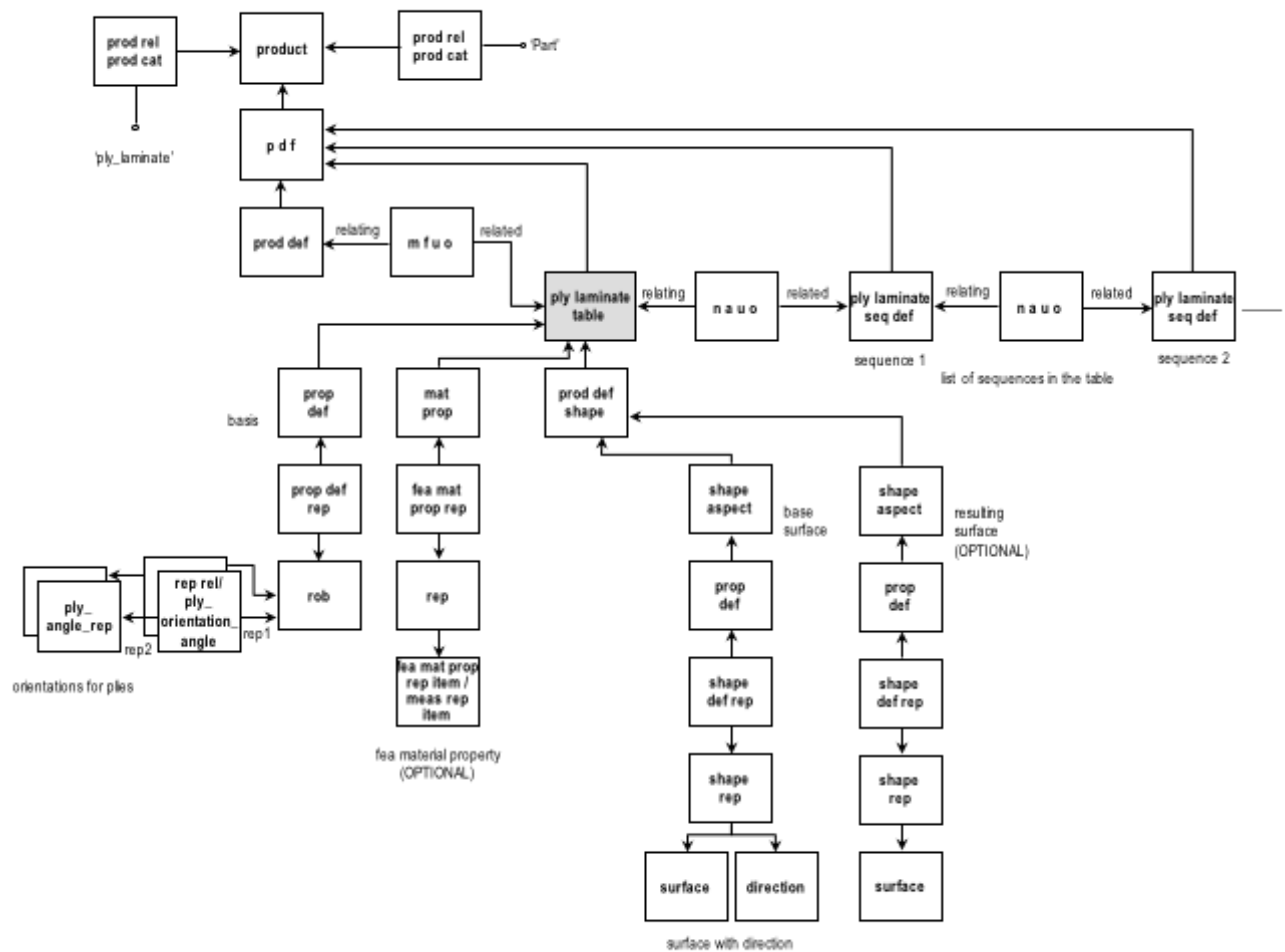
Figure 5: Ply Laminates Table
