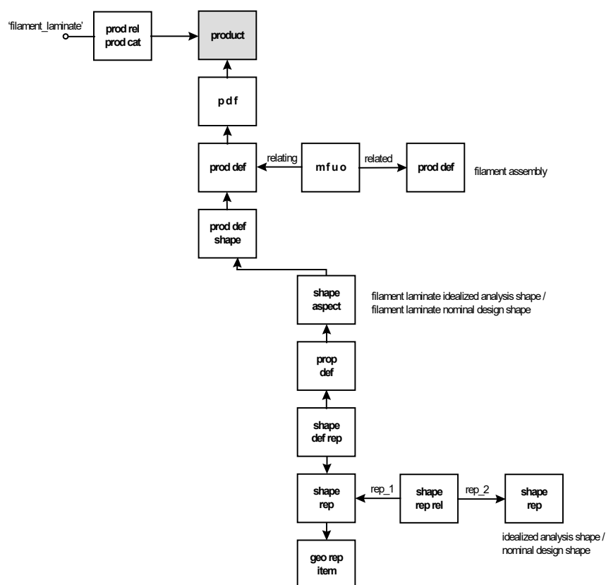
Figure 27: Filament Laminate
