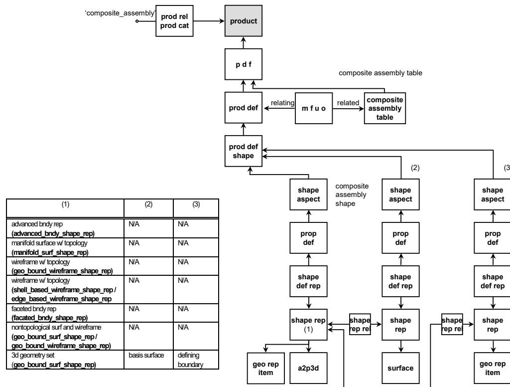
Figure 29: Composite Assembly
