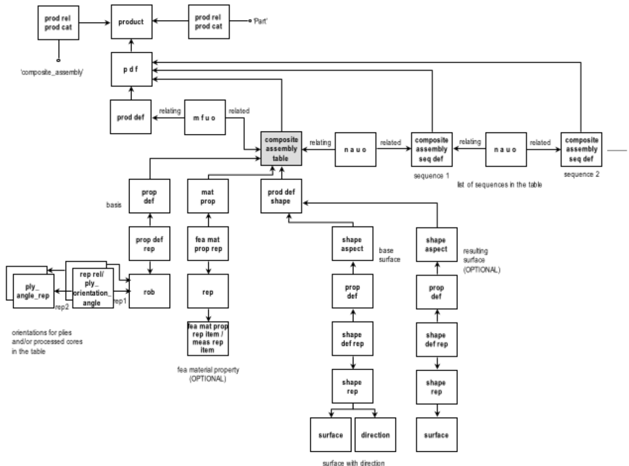
Figure 7: Composite Assembly Table
