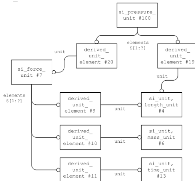
Figure 15: SI Unit Definition for "Pascal"
