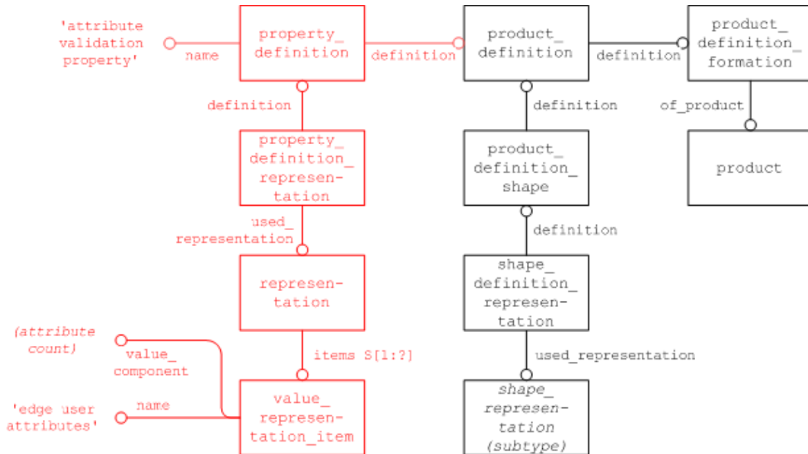
Figure 12: Definition of user defined Attribute Validation Properties
