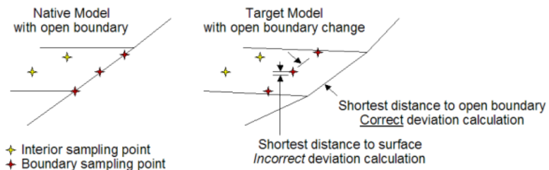
Figure 17: COPS – Sampling Points for an Open Boundary
