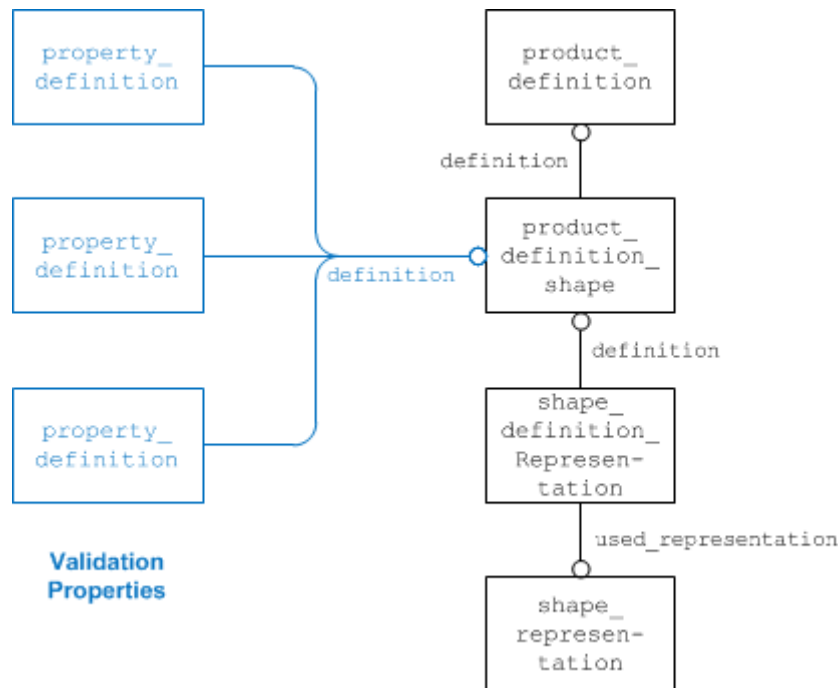
Figure 1: Validation Properties at the Part/Product level
