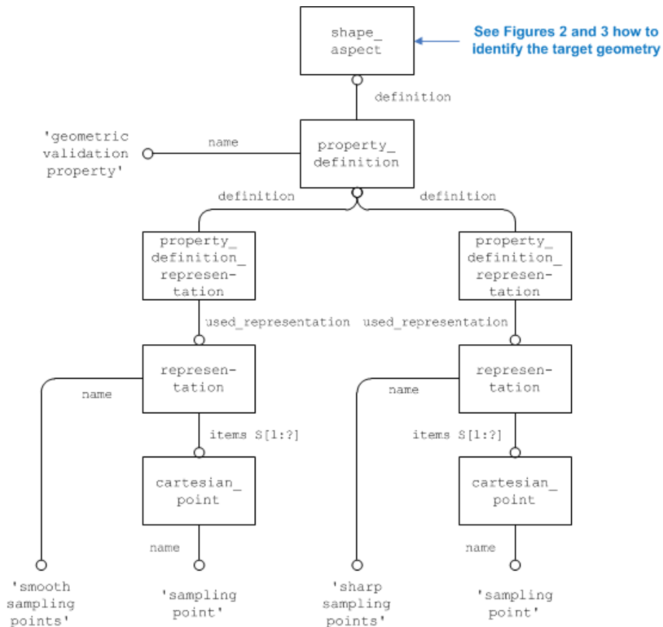
Figure 18: Cloud Of PointS Validation Property
