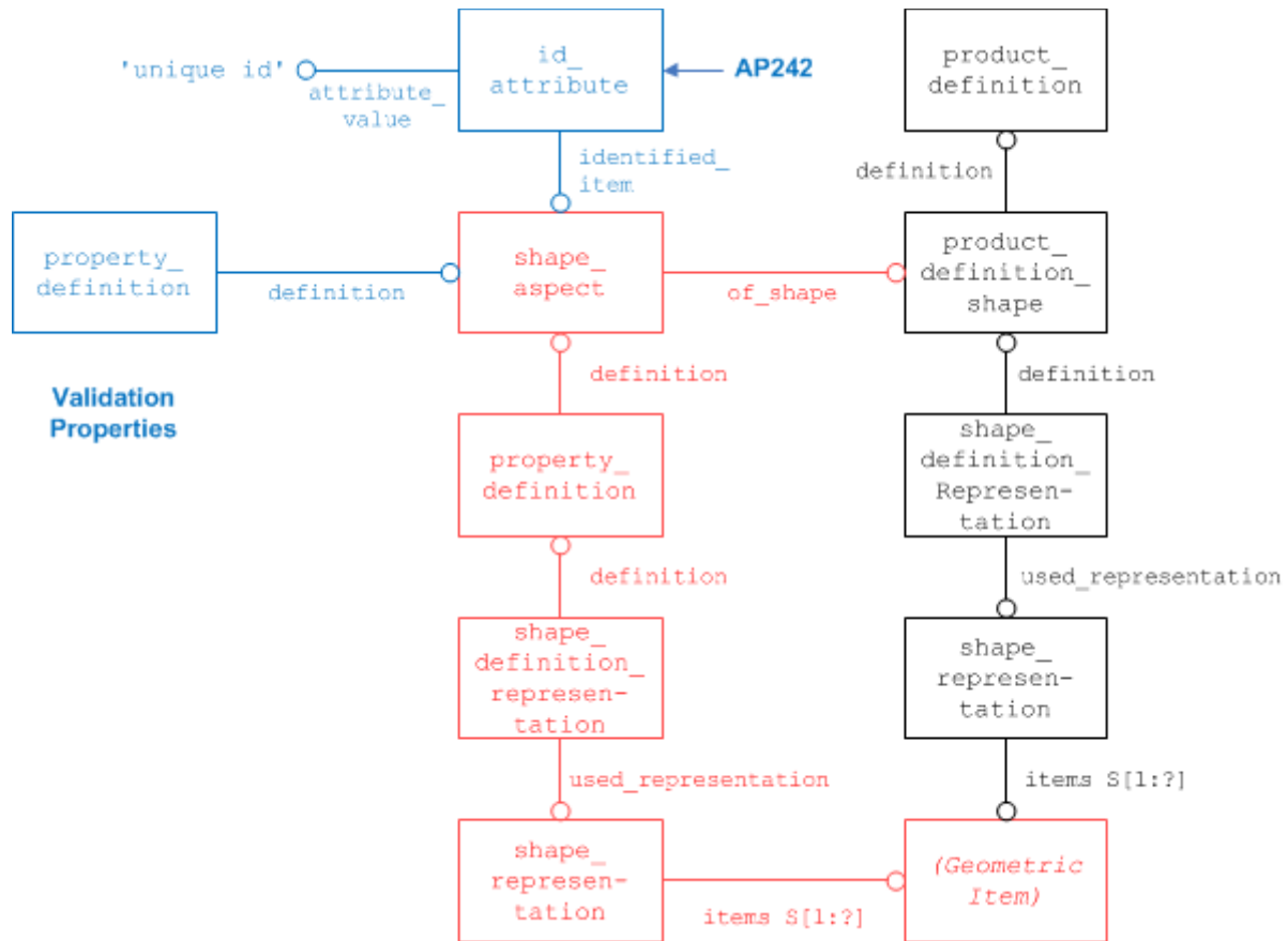
Figure 2: Validation Properties at the Geometry Level (Shape Representation)
