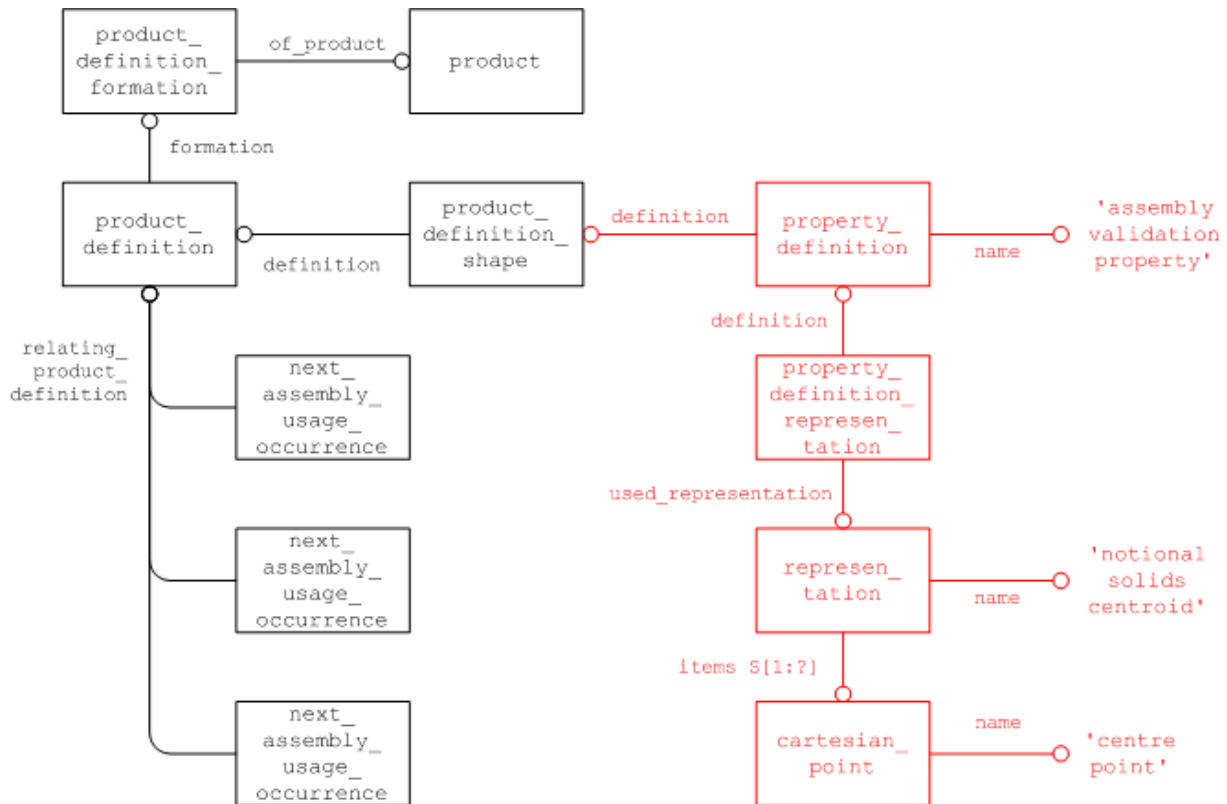
Figure 20: "Notional Solids Centroid Position" Validation Property
