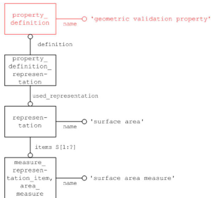
Figure 5: Geometric Validation Property "Surface Area"
