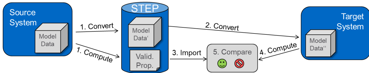
Figure 12: Validation Property Evaluation Process
