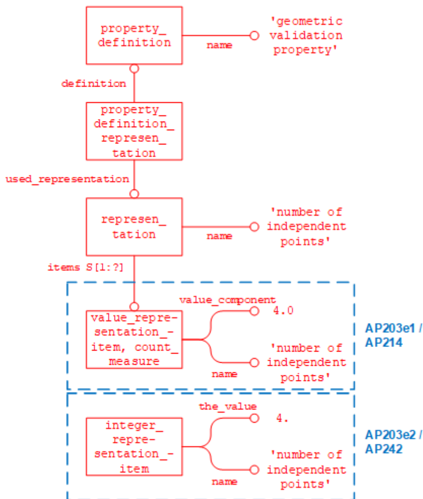
Figure 8: Geometric Validation Property “Number of Independent Points”
