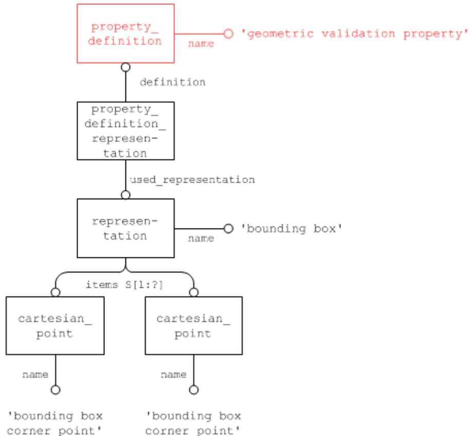
Figure 10: Geometric Validation Property "Bounding Box"
