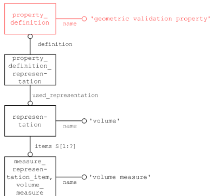
Figure 4: Geometric Validation Property “Volume”
