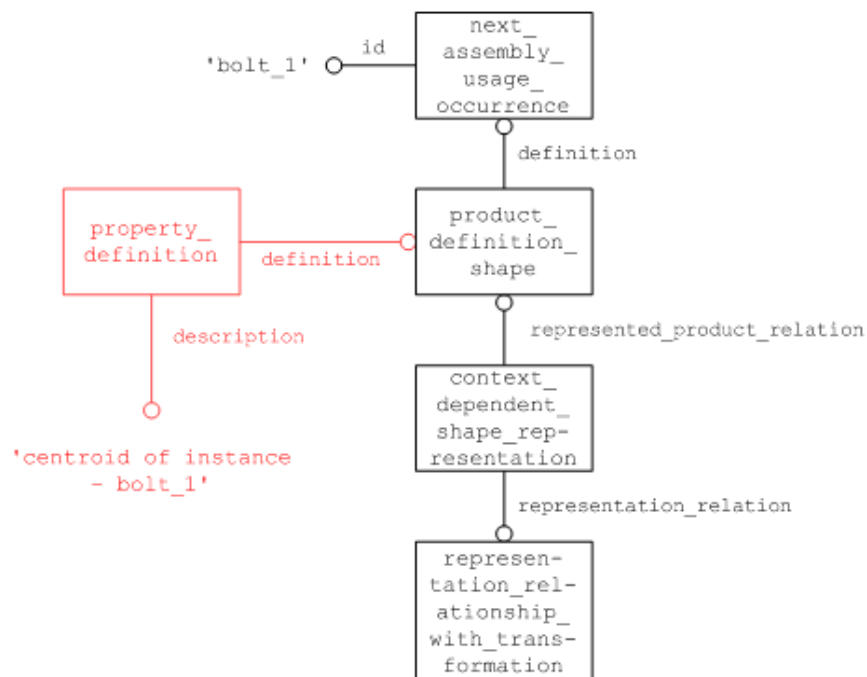
Figure 14: Extended Validation Property
