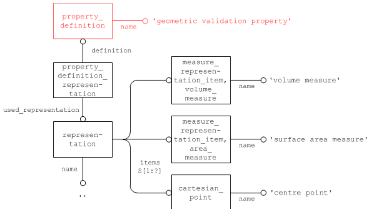
Figure 11: Combining volume, area and centroid in one property definition
