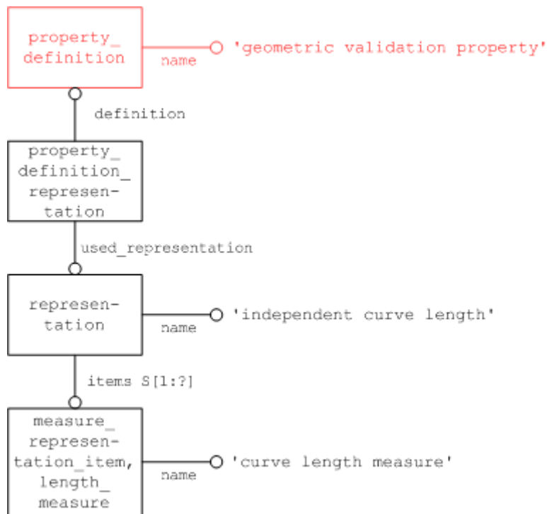
Figure 7: Geometric Validation Property “Independent Curve Length”
