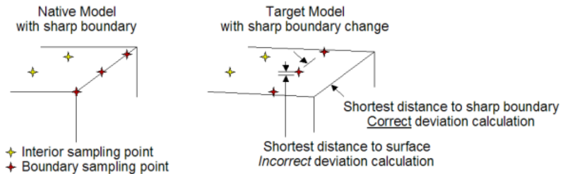
Figure 16: COPS – Sharp Sampling Points
