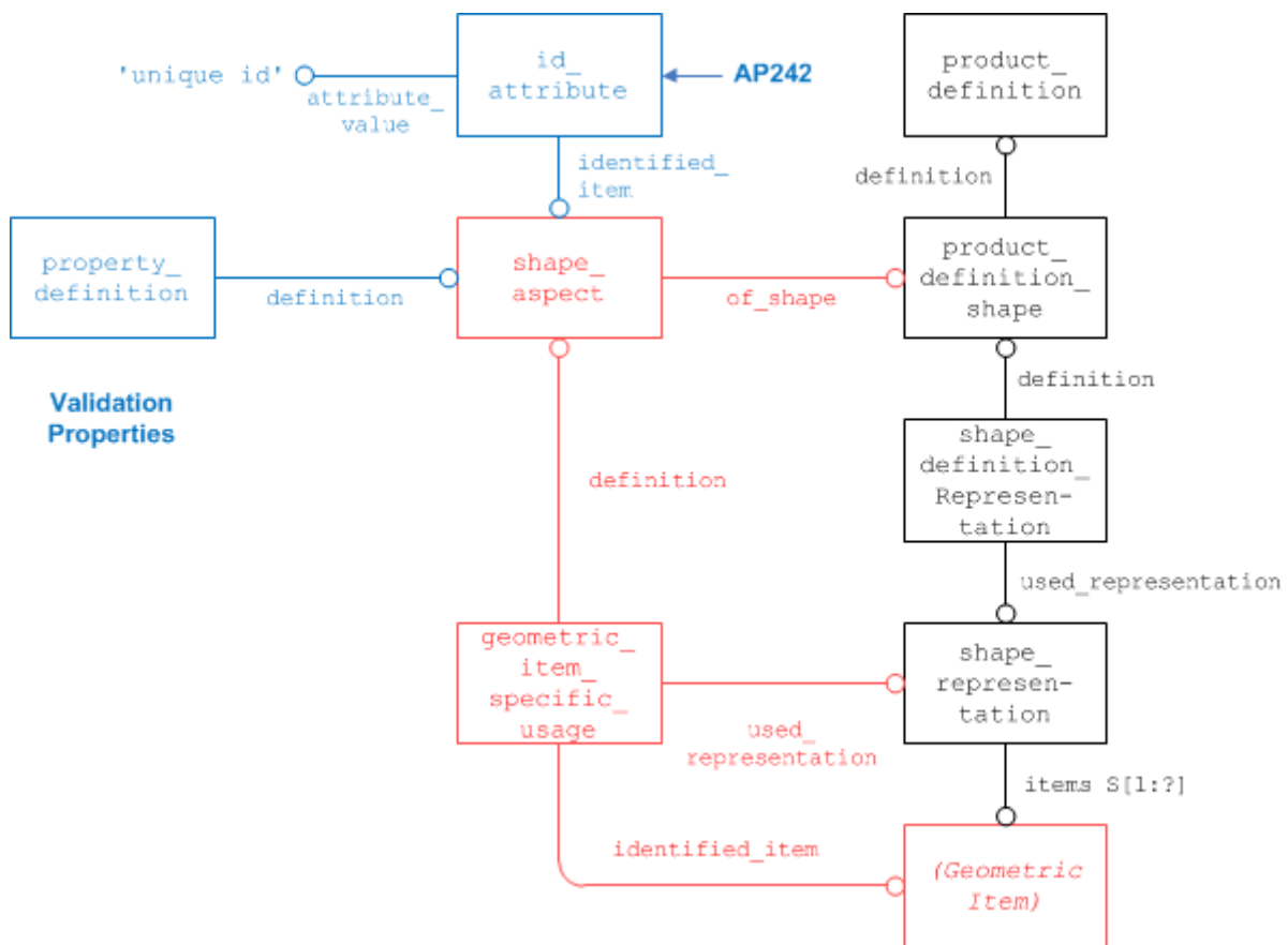
Figure 3: Validation Properties at the Geometry Level (GISU)
