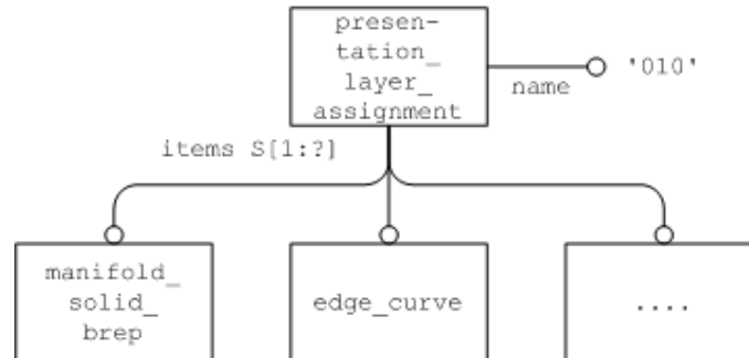
Figure 14: Layer Representation
