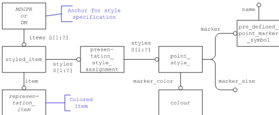
Figure 4: Definition of Point Style and Color
