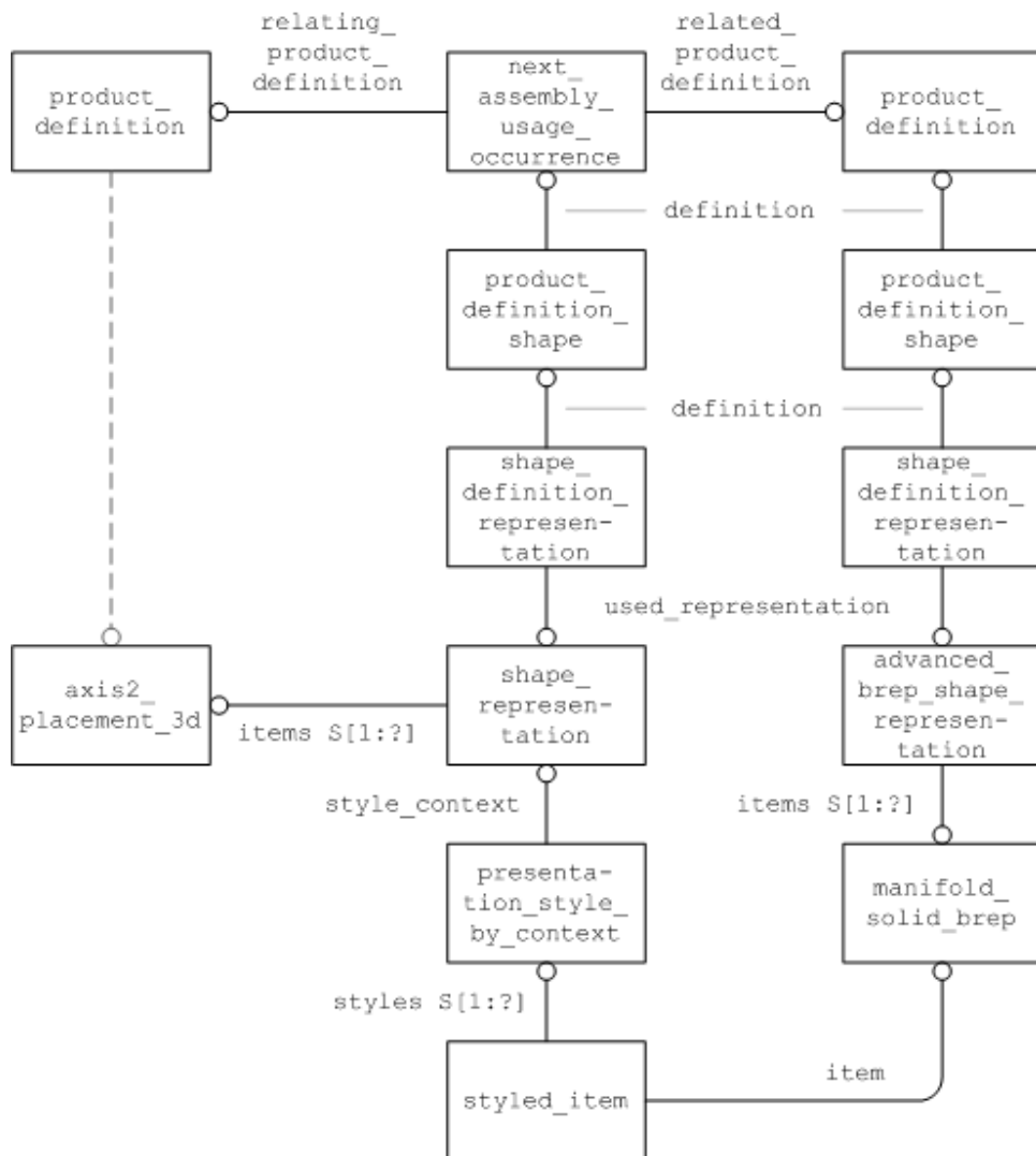
Figure 8: Structure of the Assignment of a Style to the NAUO
