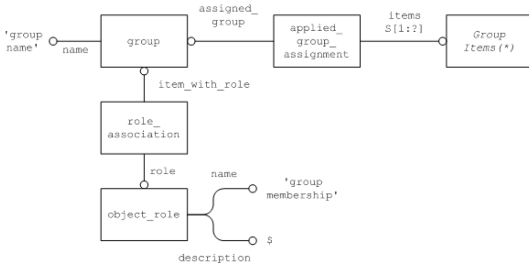
Figure 12: Group Assignment Representation
