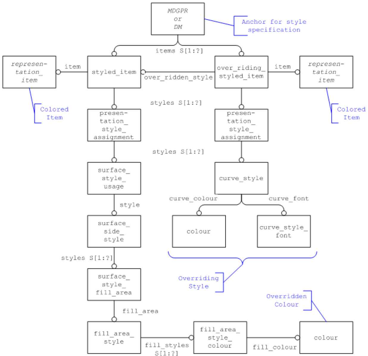
Figure 6: Representation of Overriding Edge Color
