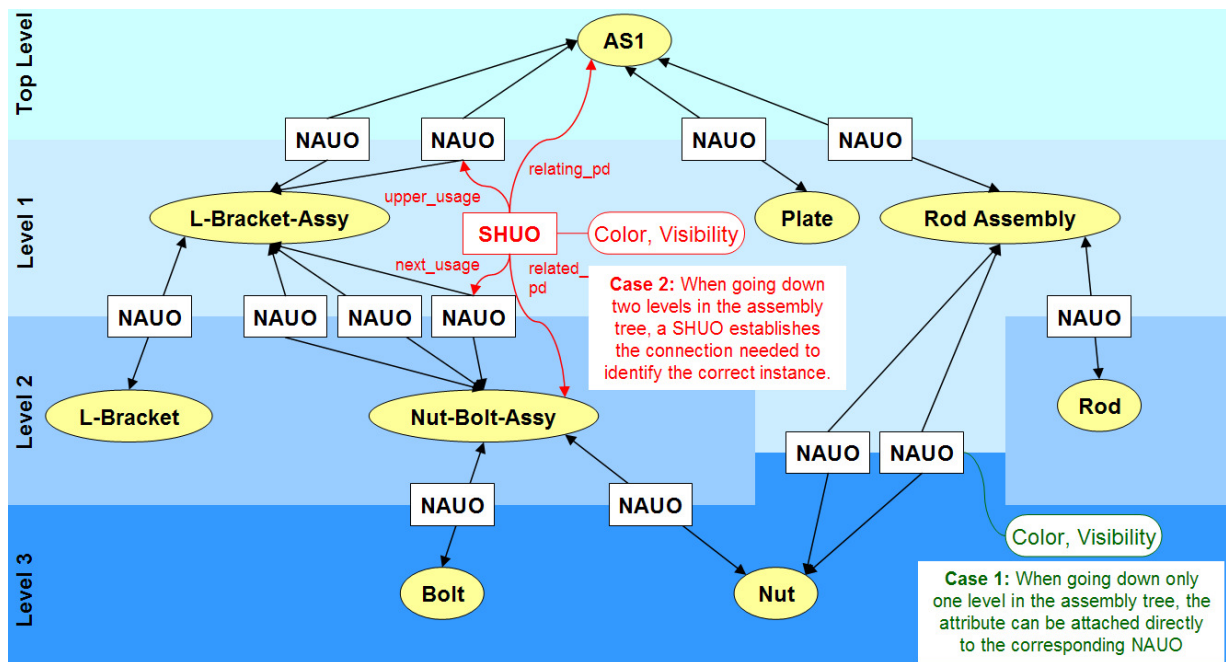
Figure 7: Identification of the Instance to be Styled
