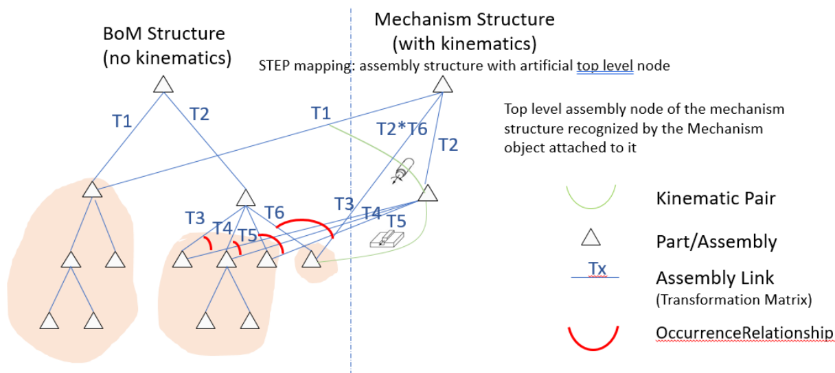
Figure 12: Complex case: use of additional assembly nodes
