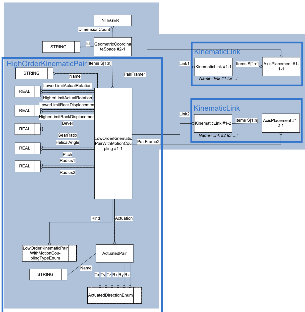
Figure 7: Template “LowOrderKinematicPairWithMotionCoupling”
