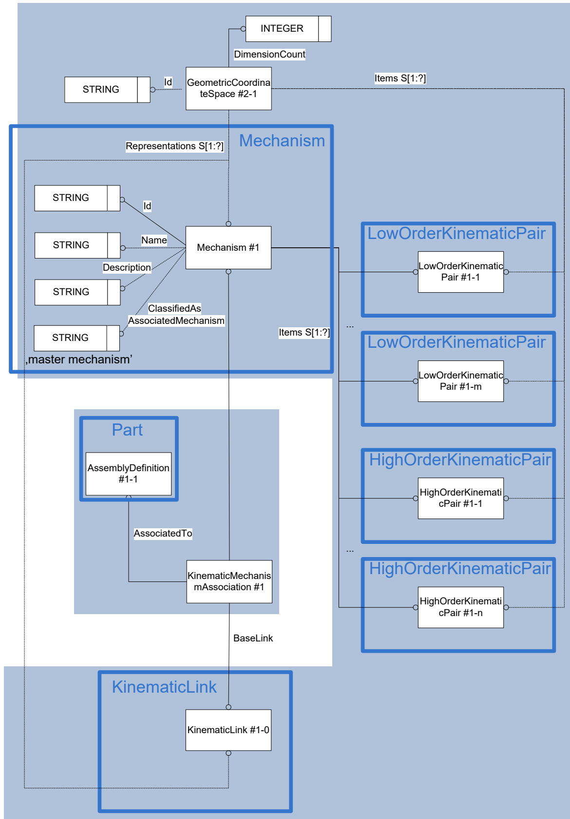
Figure 8: Template “Mechanism”
