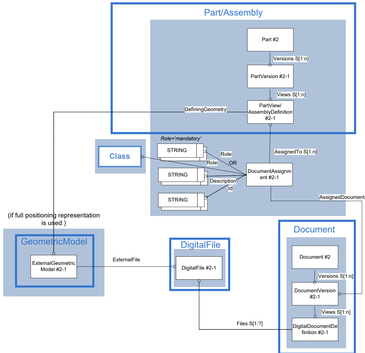
Figure 62: Template "PDM Representation for DocumentAssignment"
